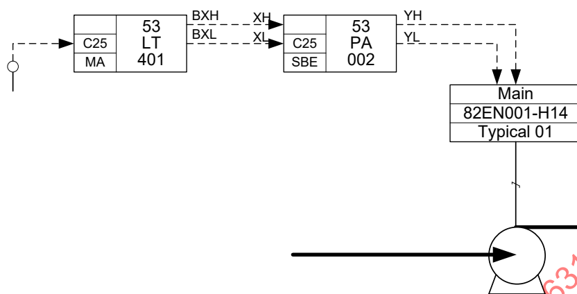
Figure E.21 – Start/Stop control of pump
