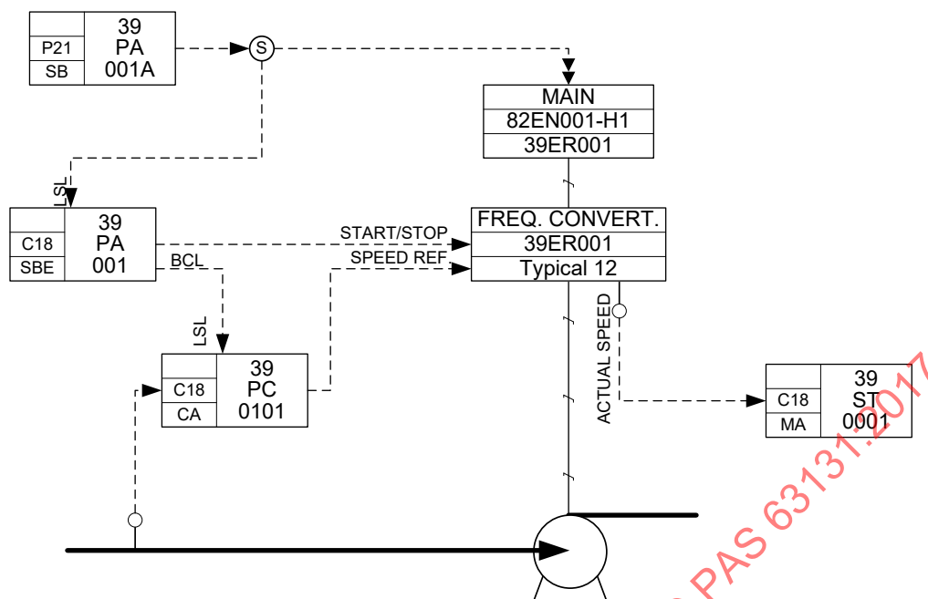
Figure E.41 – Low voltage motors with modulating control via hardwired signals
