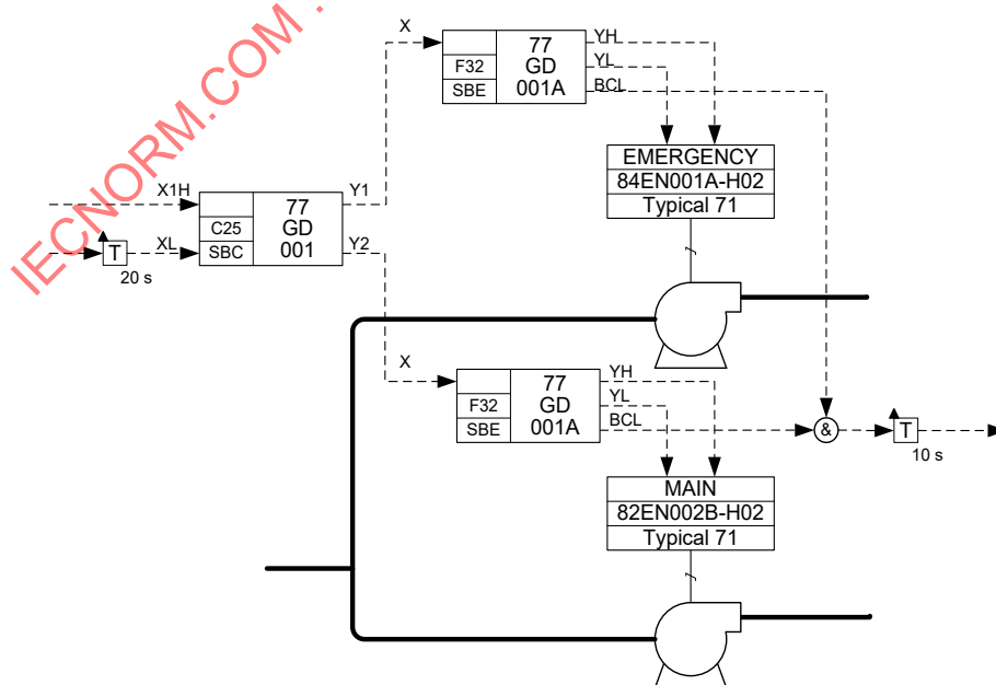
Figure E.46 – Control of multiple fans
