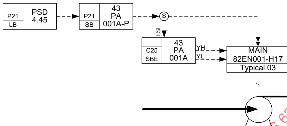
Figure E.37 – Process shutdown level safeguarding of pump
