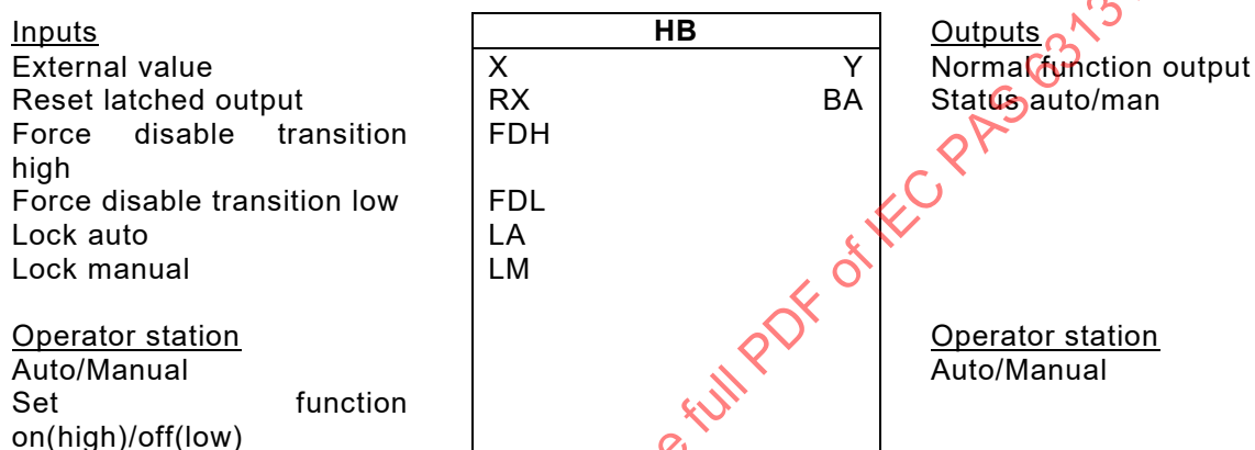
Figure A.5 – HB function template schematic I
