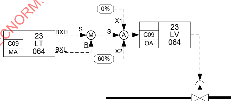
Figure E.20 – Binary control with modulating control valve
