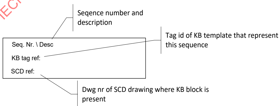
Figure B.38 – SFC sequence start and reference symbol
