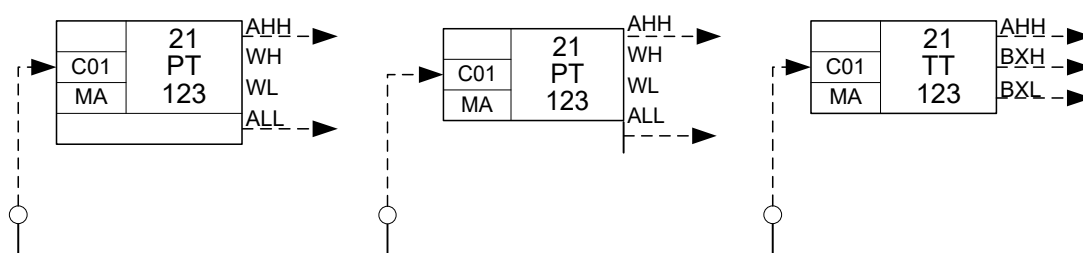
Figure E.1 – MA terminals
