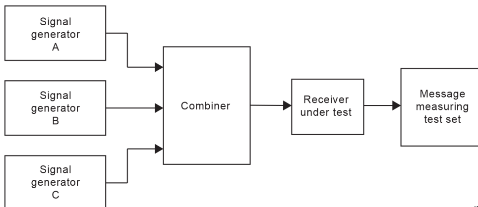
Figure 13 – Measurement arrangement for intermodulation
