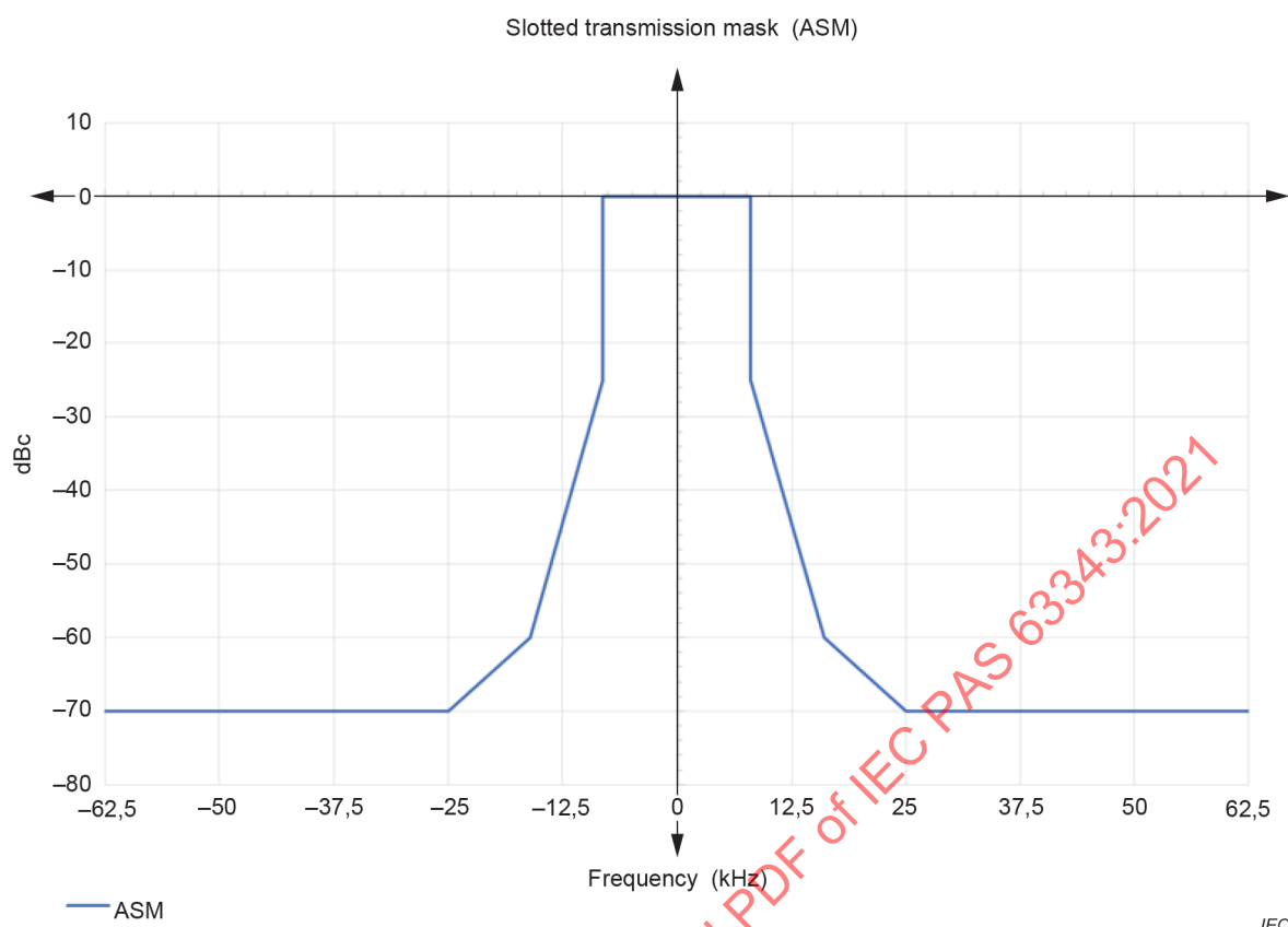
Figure 4 – Slotted transmission spectrum for ASM
