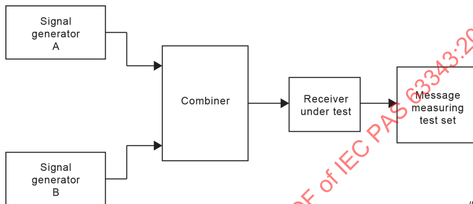
Figure 14 – Measurement arrangement for blocking or de-sensitisation
