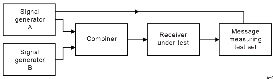
Figure 12 – Test setup for adjacent channel selectivity
