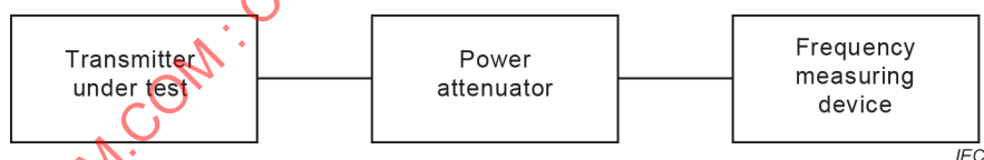
Figure 7 – Test setup for frequency error measurement
