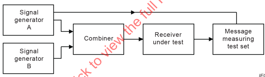
Figure 8 – Test setup for adjacent channel selectivity
