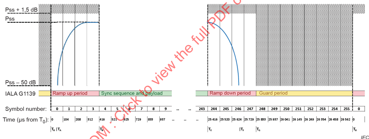
Figure 2 – Transmitter power versus time characteristics for \pi/4 QPSK (ASM)
