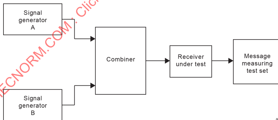
Figure 10 – Measurement arrangement for blocking or de-sensitisation
