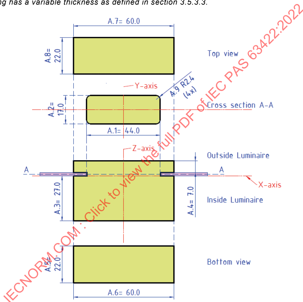
Figure 3-3 – Demarcation model for the LEX-M – category R44x17
