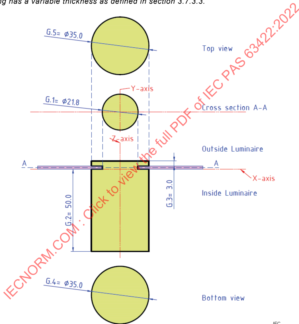
Figure 3-9 – Demarcation model for the LEX-M – category C22-T1
