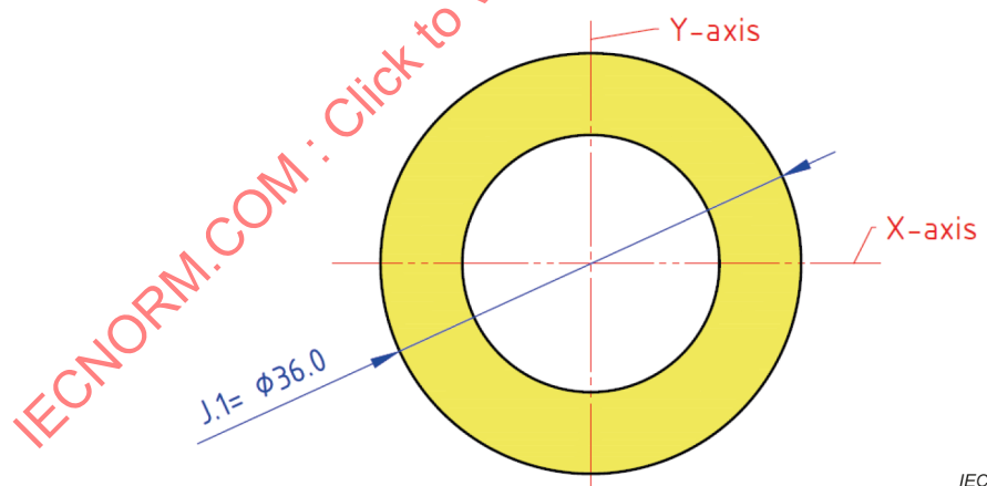
Figure 3-14 – Border of the LEX-S – category C22-T2
