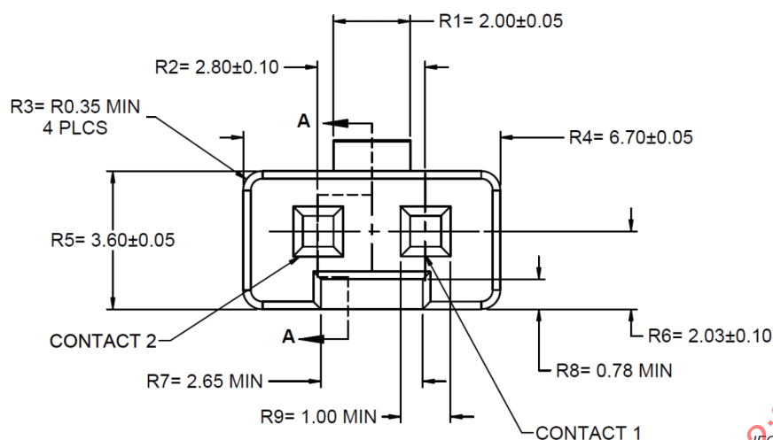
Figure 3-23 – Mechanical interface of the mating area of the LEX-LP
