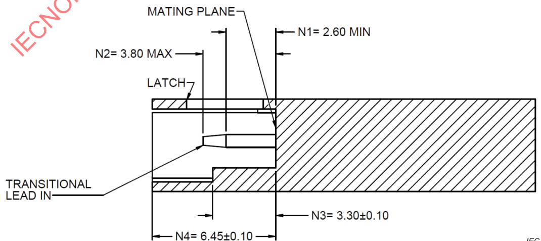
Figure 3-19 – Mechanical interface of the mating area of the LEX-MR – cross section A-A
