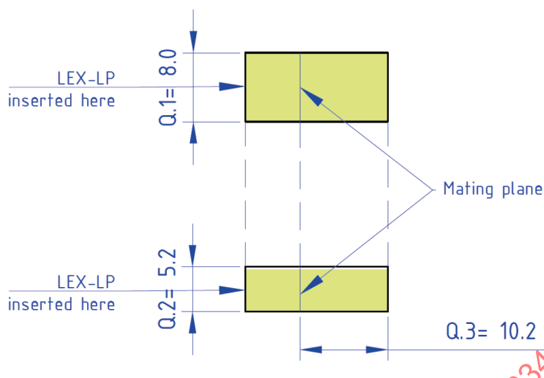
Figure 3-21 – Demarcation model of the LEX-MR (top view and side view) – wire-to-board type
