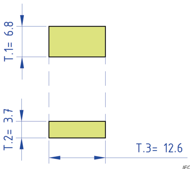
Figure 3-25 – Demarcation model of the LEX-LP (top view and side view)
