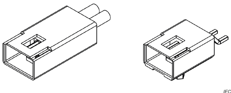
Figure 3-17 – Examples of the wire-to-wire LEX-MR and the wire-to-board LEX-MR (informative)
