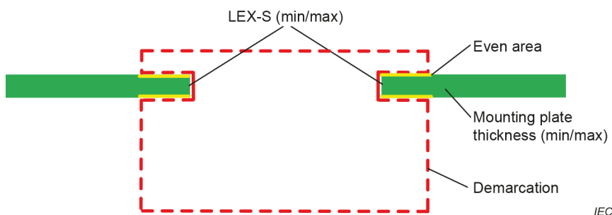
Figure 3-2 – Method of specification of the mechanical interface of the Luminaire and the LEX-M
