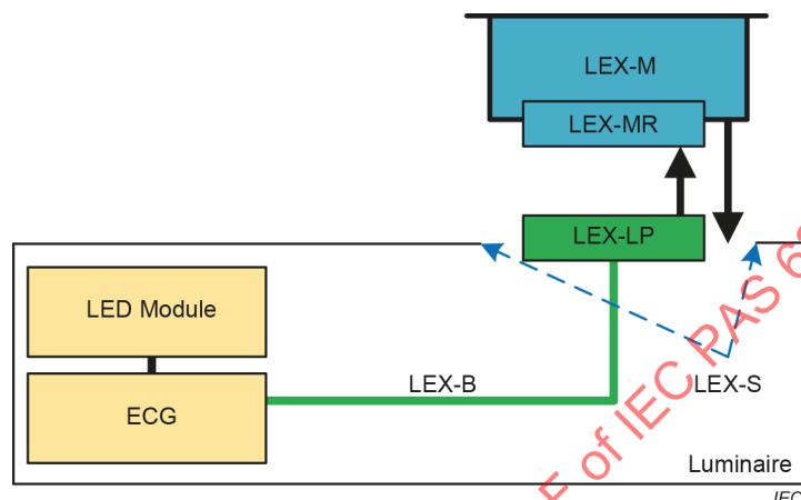
Figure 2-1 – Schematic overview of a typical Book 20 Luminaire and a Luminaire Extension Module
