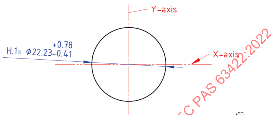
Figure 3-13 – Dimensions of the LEX-S – category C22-T2
