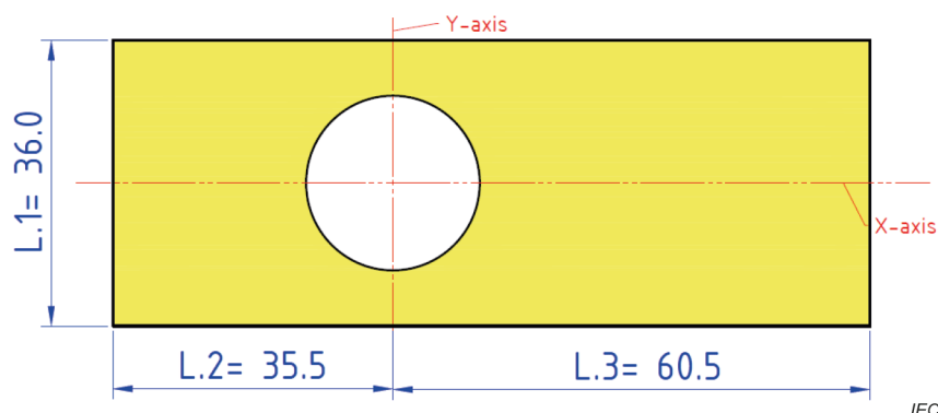
Figure 3-15 – Internal border of the LEX-S – category C22-T2
