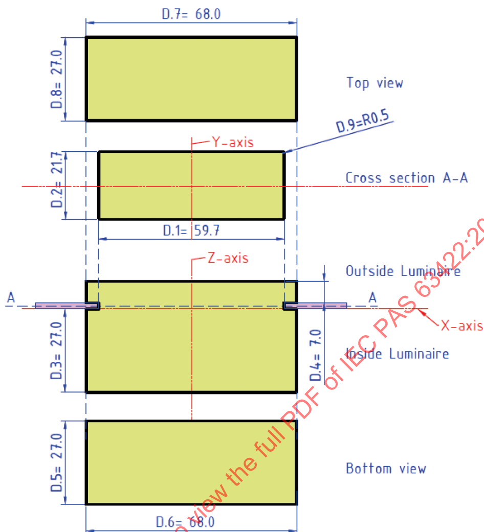
Figure 3-6 – Demarcation model for the LEX-M – category R60x22
