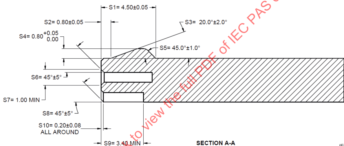
Figure 3-24 – Mechanical interface of the mating area of the LEX-LP – cross section A-A
