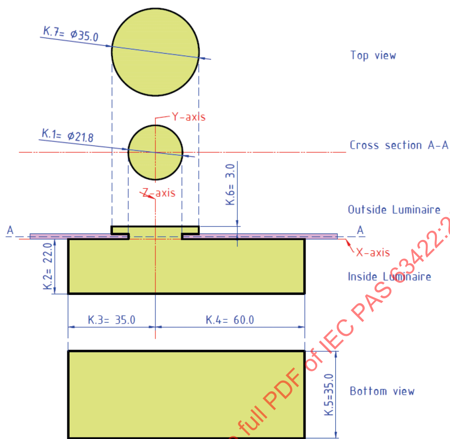
Figure 3-12 – Demarcation model for the LEX-M – category C22-T2
