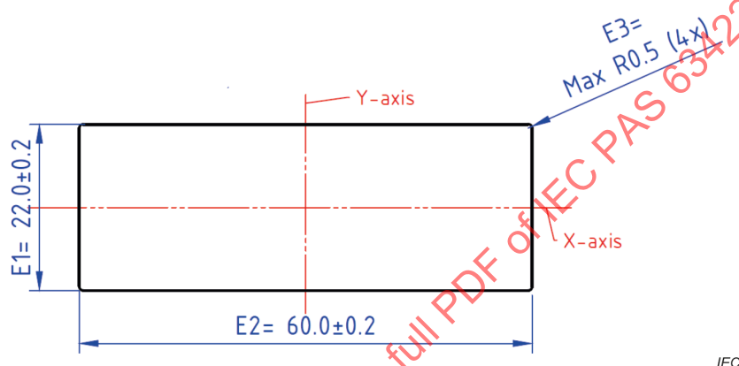
Figure 3-7 – Dimensions of the LEX-S – category R60x22
