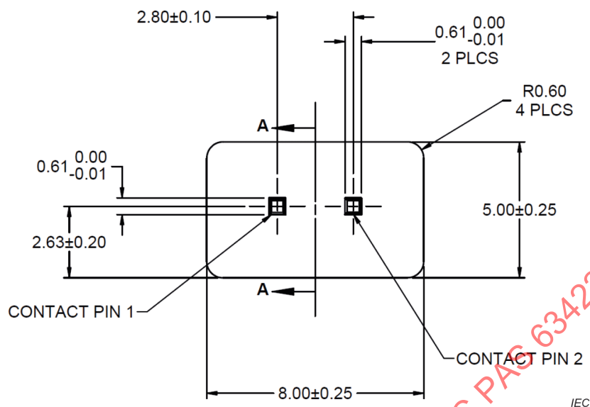
Figure 5-3 – Mechanical interface of the mating area of the LEX-LP GO-Gauge
