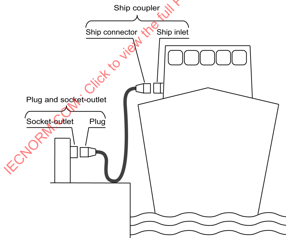
Figure 5 – Diagram showing the use of accessories
