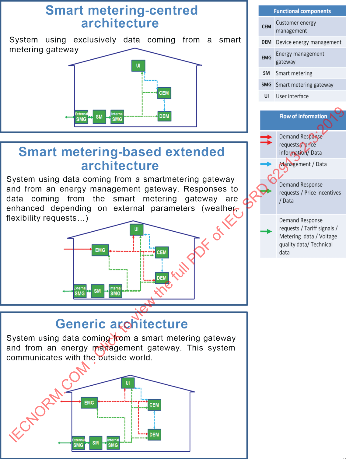
Figure A.3 – France – COSEI architectures
