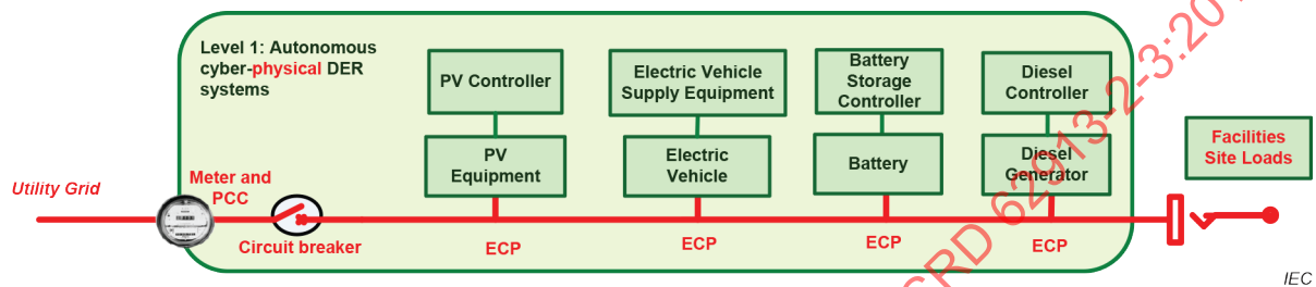
Figure B.1 – Level 1 DER systems with autonomous functions at facility and DSO sites
