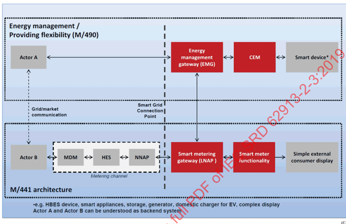
Figure A.2 – EU M/490 – Flexibility Functional Architecture (CEN-CENELEC-ETSI)
