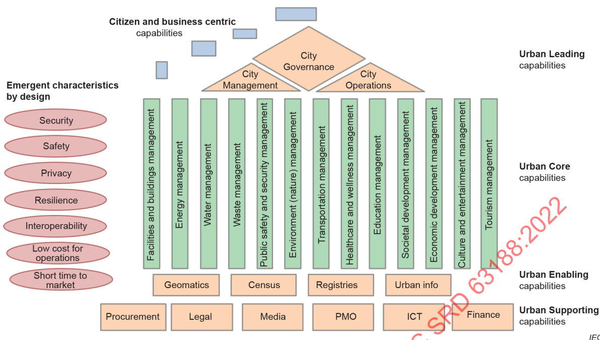
Figure 31 – Potential SCRA level 1 reference capability map
