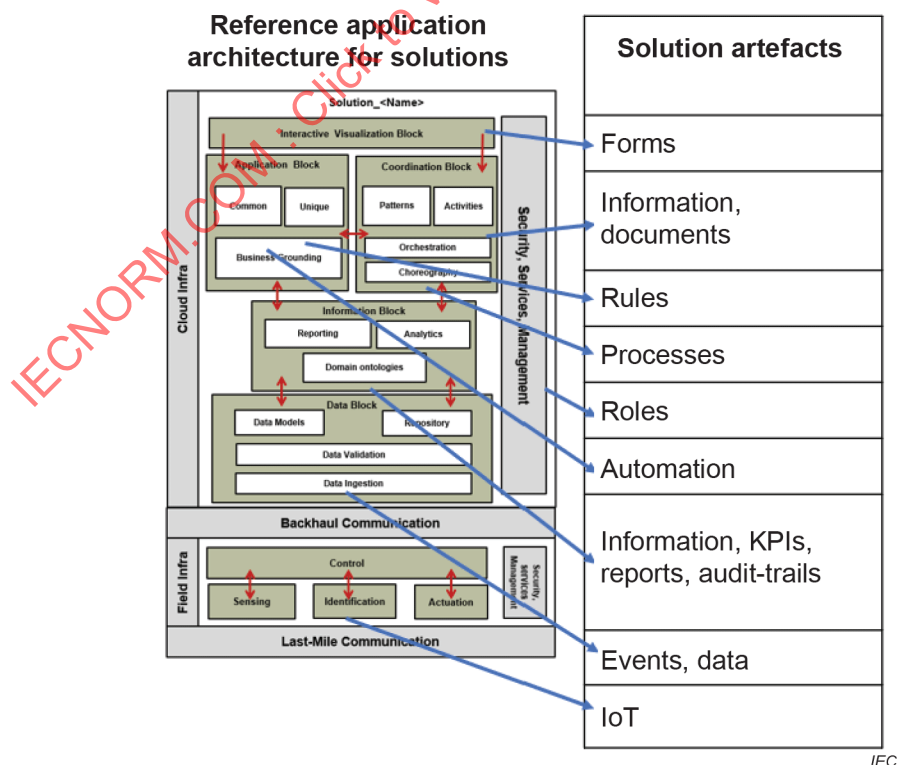
Figure 19 – Reference application architecture for solutions
