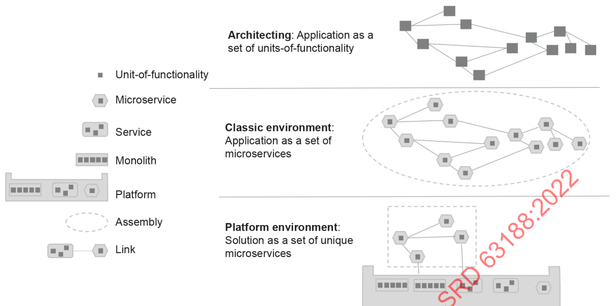
Figure 17 – Using together services, microservices and monoliths
