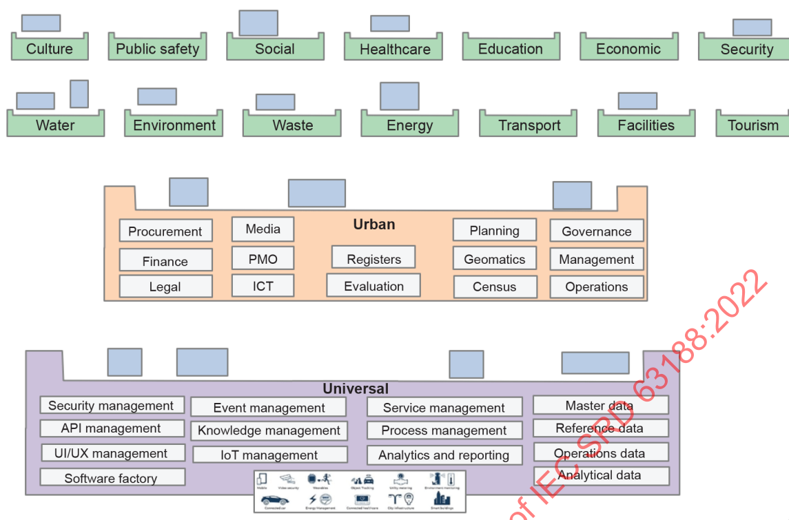
Figure 16 – An example of Common Smart Cities Digital Repeatabl Platform structure
