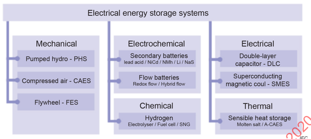
Figure 3 – Classification of electrical energy storage systems according to energy form
