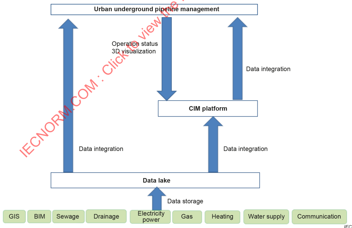
Figure 14 – Positioning city information modelling in urban underground pipeline management
