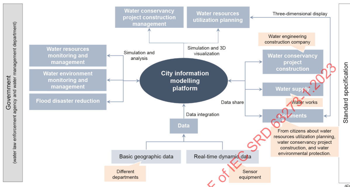
Figure 12 – Positioning city information modelling structure in water management
