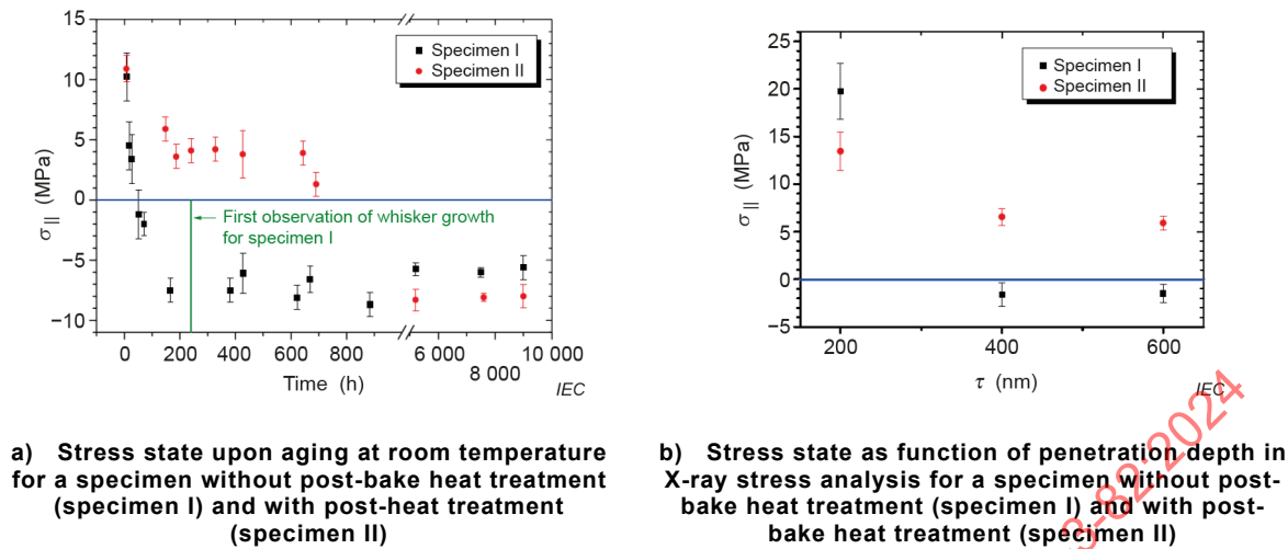
Figure 10 – Stress states of different Sn surface finishes [16]
