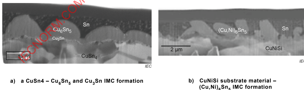
Figure 12 – IMC formation of Sn surface finishes
