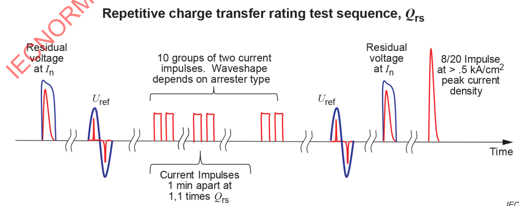
Figure 3 – Sequence of the test to verify the repetitive charge transfer rating
