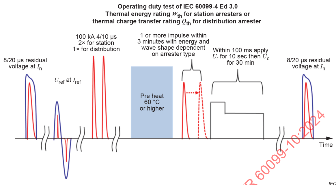
Figure 5 – Operating duty test sequence
