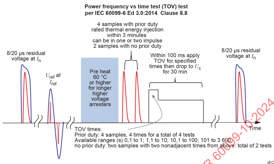
Figure 7 – Power-frequency versus time test sequence
