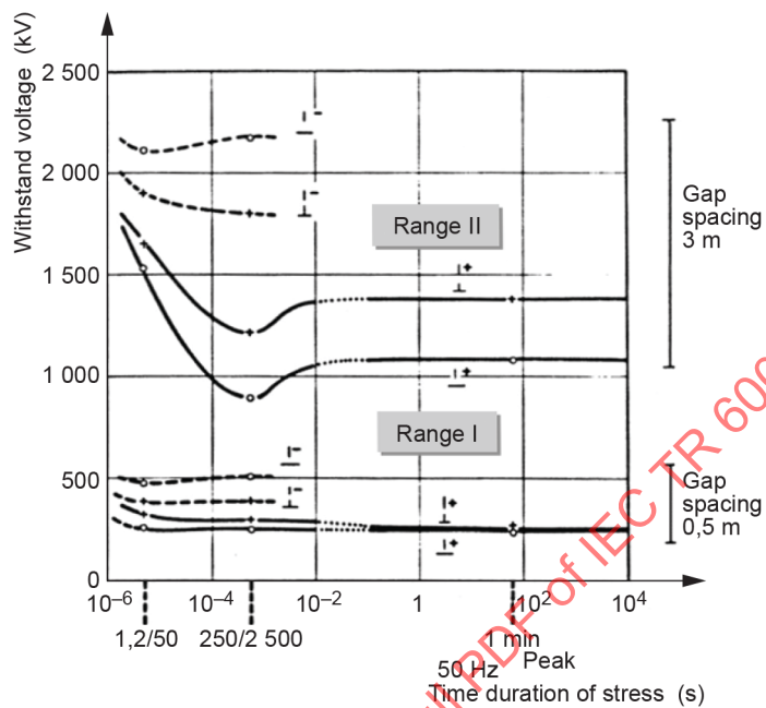
Figure 2 – Withstand voltage versus duration
