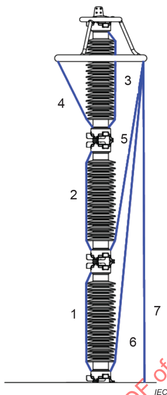
Figure 1 – Possible arcing distances (7 paths to consider for this example) for a multi-unit arrester (from CIGRÉ 696-2017)
