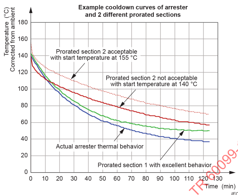
Figure 4 – Example of cooldown curves of test samples
