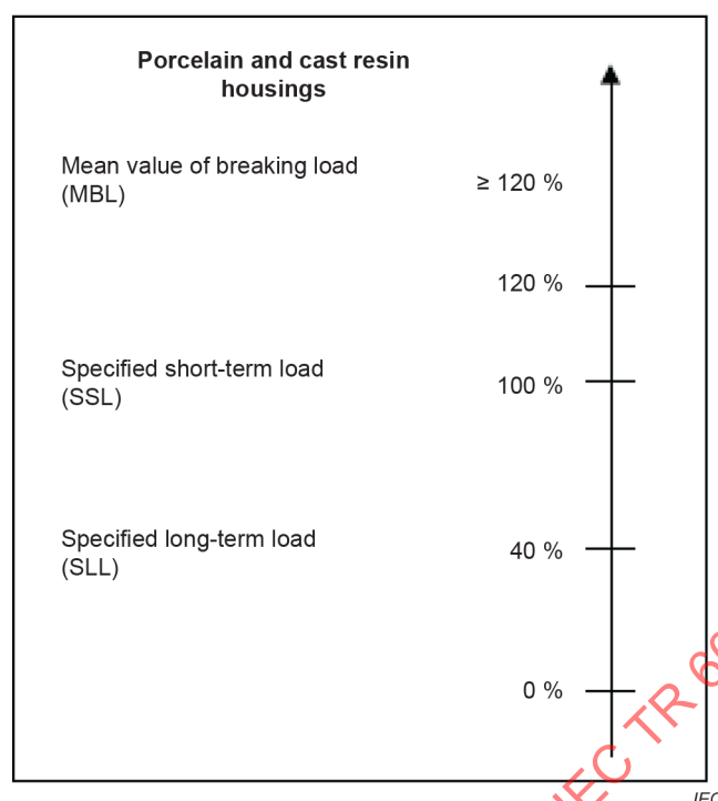
Figure 9 – Graphic representation of the relationships between tests in the bending moment tests for porcelain-housed arresters
