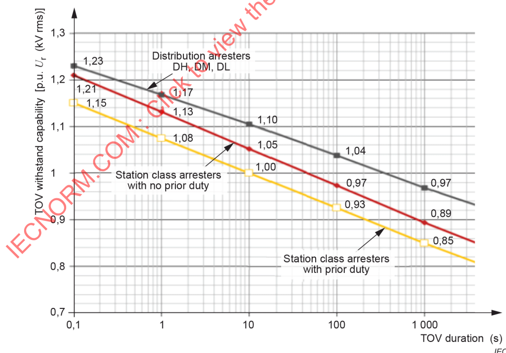
Figure 6 – Examples of TOV curves
