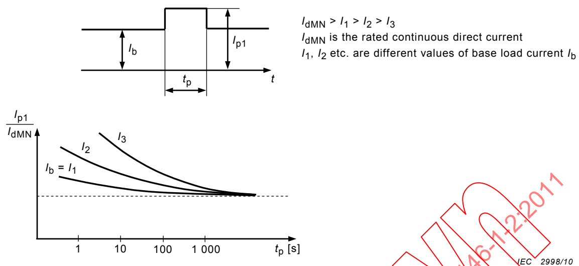
Figure 13 – Single peak load
