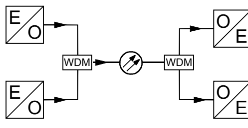
Figure 4 – Real wavelength division multiplex system
