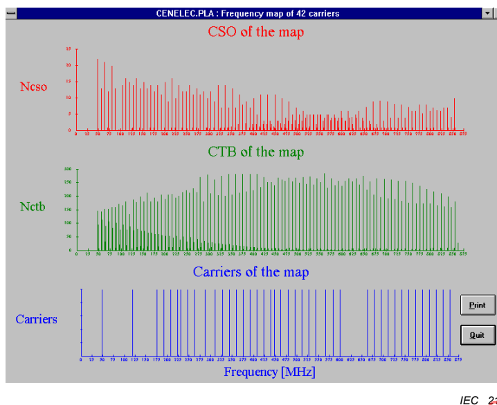
Figure C.2 – Weighted second- and third-order distortion repartition for the 42 carriers frequency allocation map defined in Table C.1 of IEC 60728-3 (software window capture)
