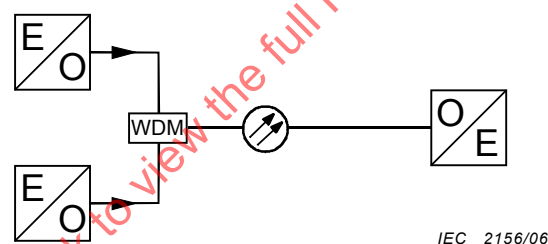
Figure 3 – Multipoint-to-point system
