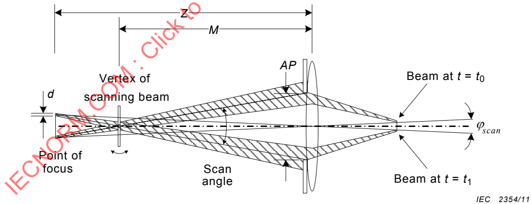
Figure 13 – Imaging a scanning apparent source located beyond the scanning beam vertex
