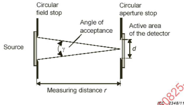
Figure 8b – Measurement set-up for accessible source
