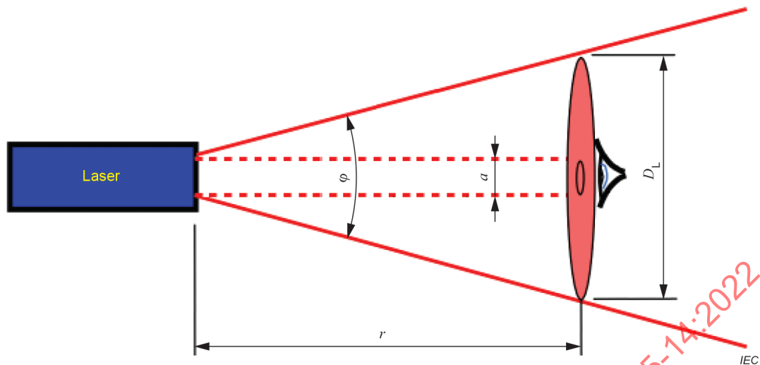
Figure B.1 – Nominal ocular hazard distance
