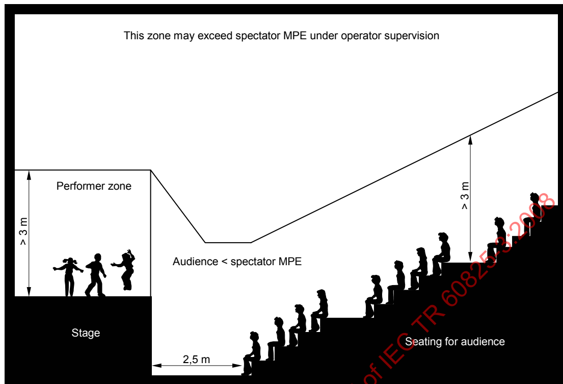
Figure 3 – Audience/spectator separation with operator in control
