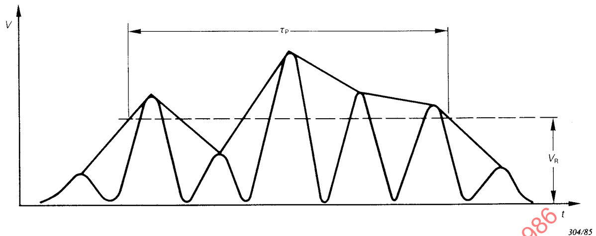
FIG. 1. — Illustration of the procedure for determining echo pulse duration \tau_p from a video A-mode display trace, as described in Sub-clause 8.2. V_R is the echo reference level referred to in the text.
