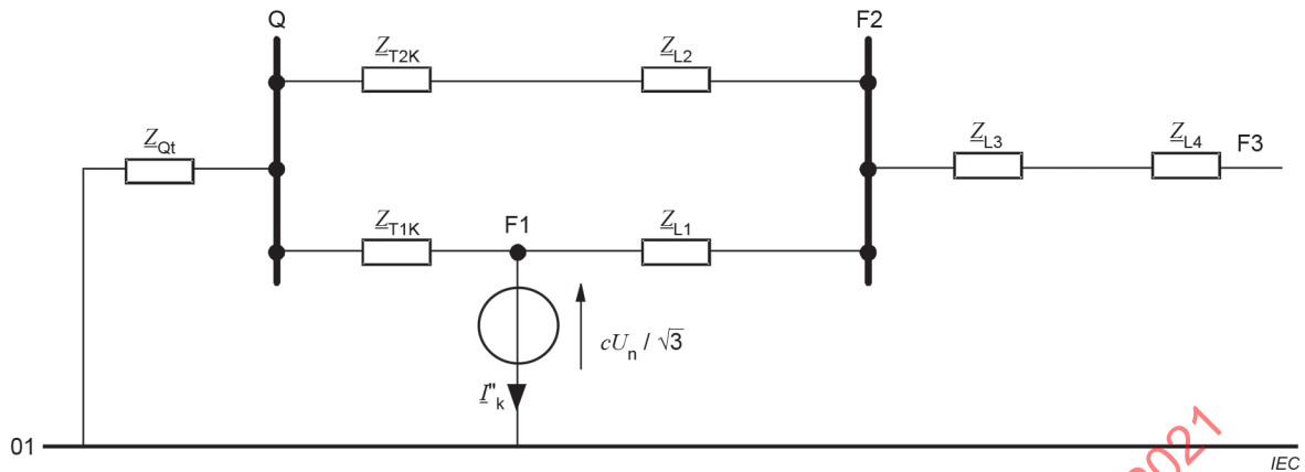
Figure 7 – Positive-sequence system (according to Figure 6) for the calculation of I_k'' at the short-circuit location F1
