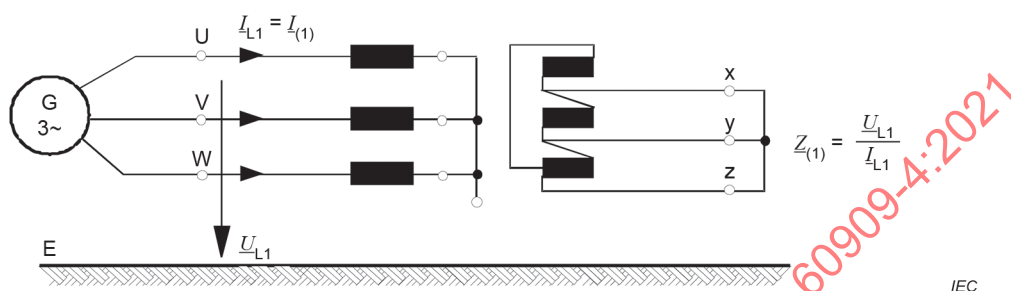
b) Positive-sequence and negative-sequence impedance Z_{(1)} = Z_{(2)}
