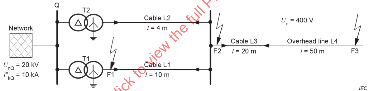
Figure 6 – Low-voltage system U_n = 400 \text{ V} with short-circuit locations F1, F2, F3
