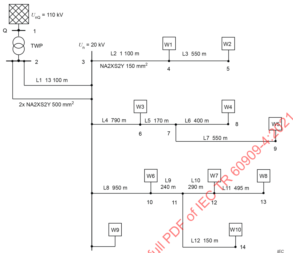
Figure 16 – Windfarm with ten wind power station units
