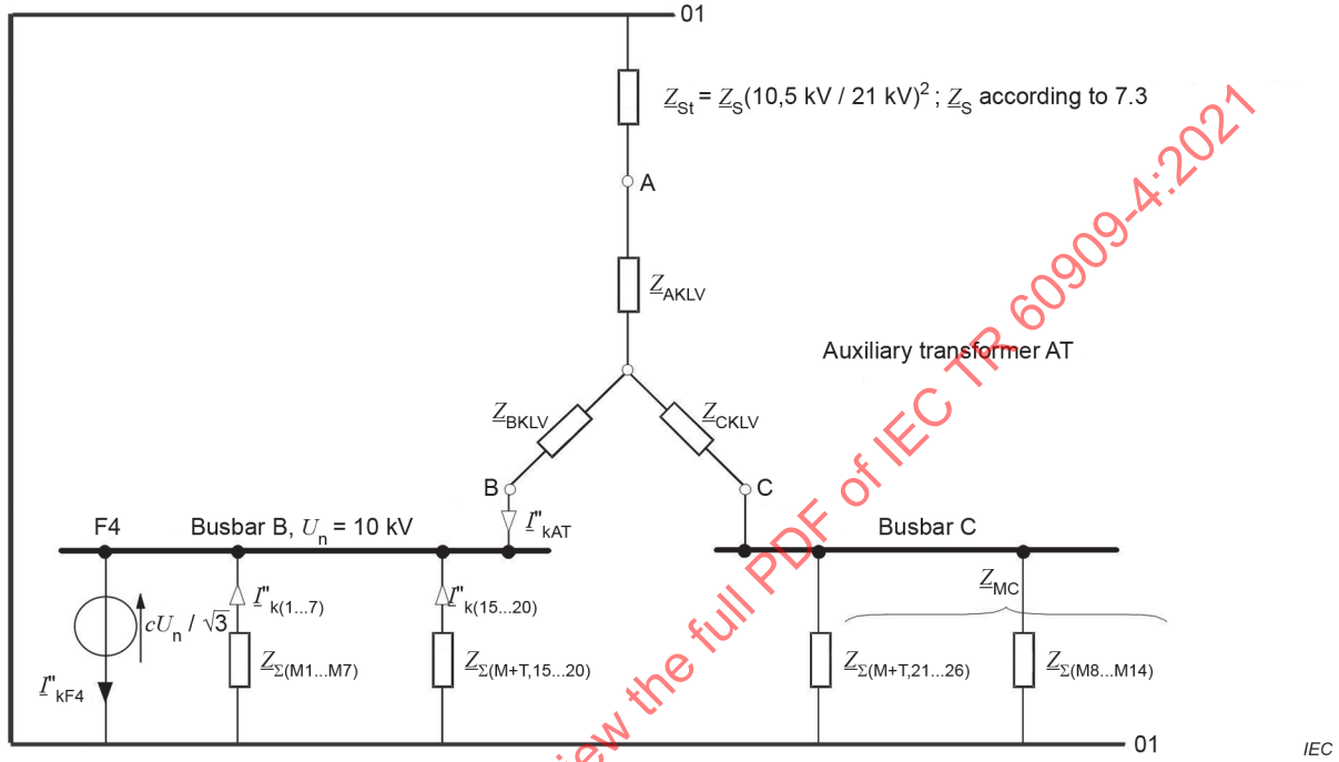
Figure 14 – Positive-sequence system for the calculation of the short-circuit currents at the location F4 (see Figure 12)
