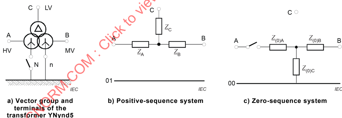
Figure 4 – Equivalent circuits of a three-winding network transformer
