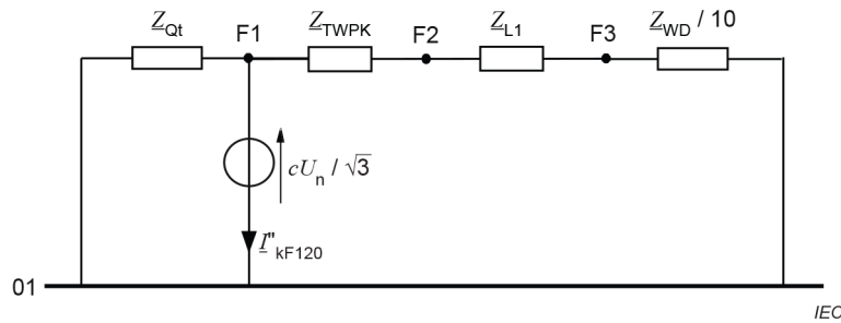
Figure 17 – Equivalent circuit diagram for the calculation of the short-circuit current at the location F1 without the consideration of the internal wind power plant cables (values are related to the 20 kV voltage level), variant 1
