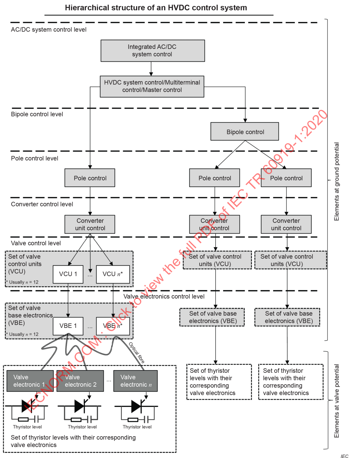
Figure 20 – Control hierarchy for HVDC/UHVDC system
