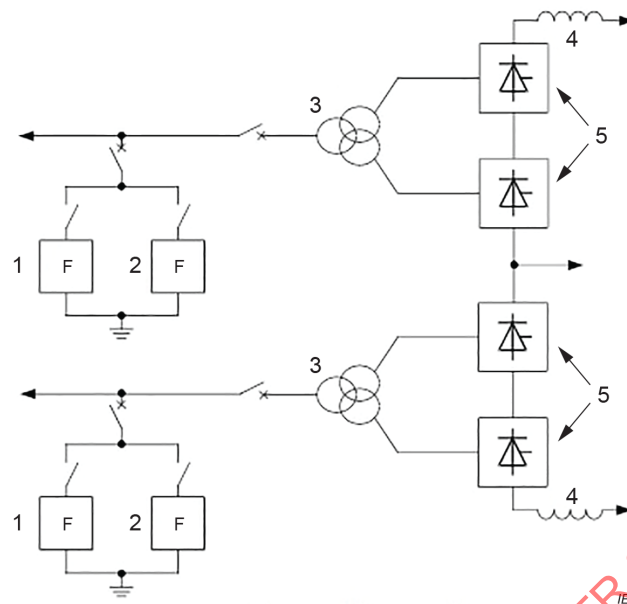
a) Separate AC system buses
