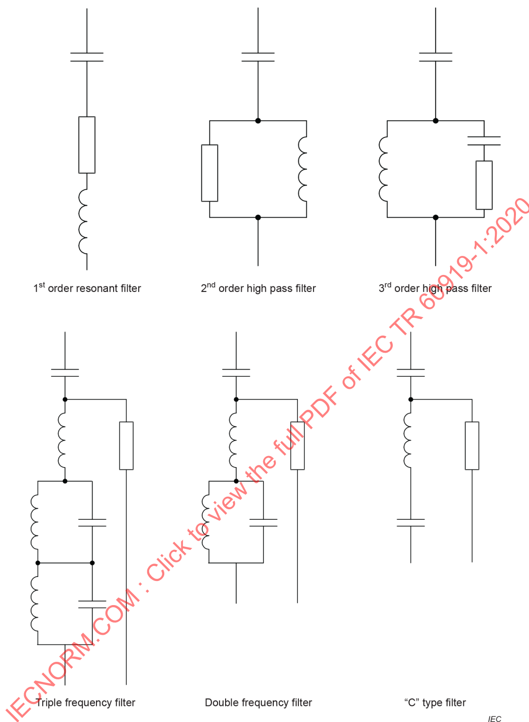
Figure 23 – Circuit diagrams for different filter types
