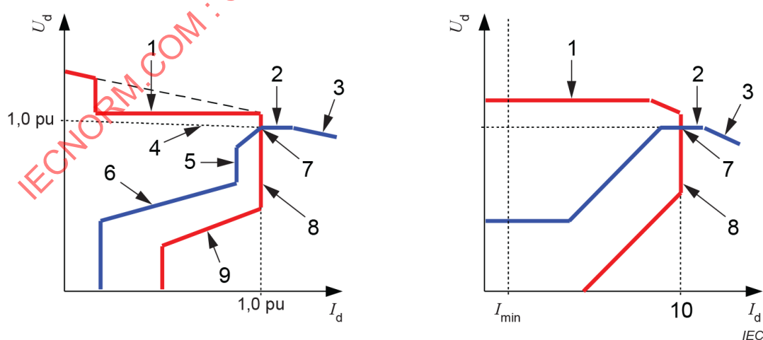
c) Examples of HVDC control characteristic
