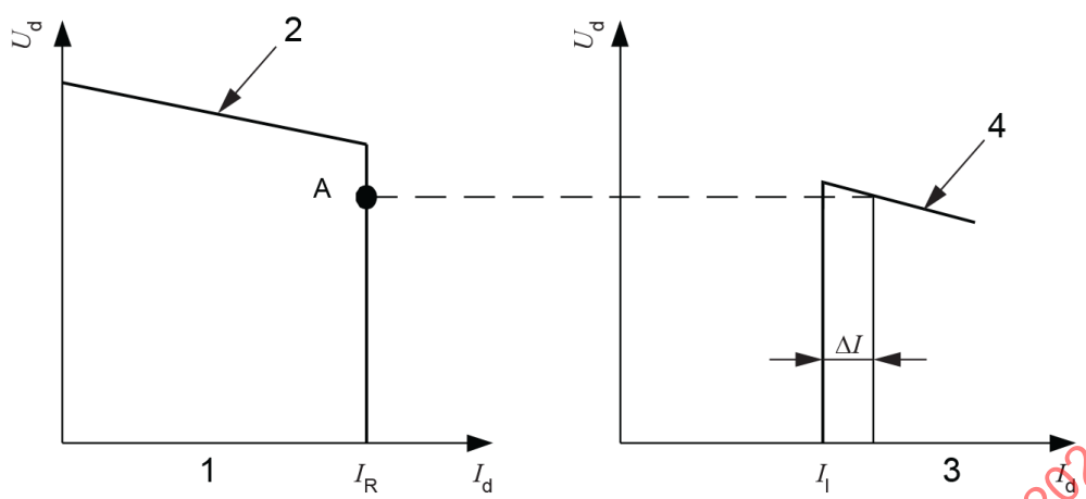
a) Normal operation, rectifier controls the current
