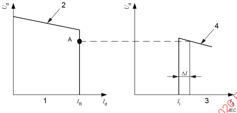
a) Normal operation, rectifier controls the current
