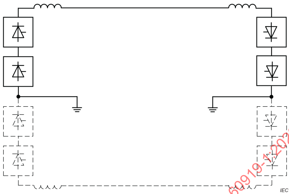
a) Monopolar to bipolar extension
