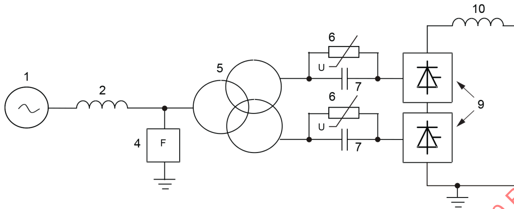
a) Capacitor commutated converter (CCC)
