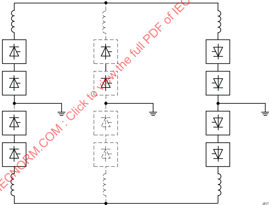
b) Multiterminal bridge extension
