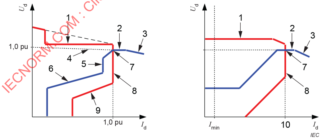
c) Examples of HVDC control characteristic
