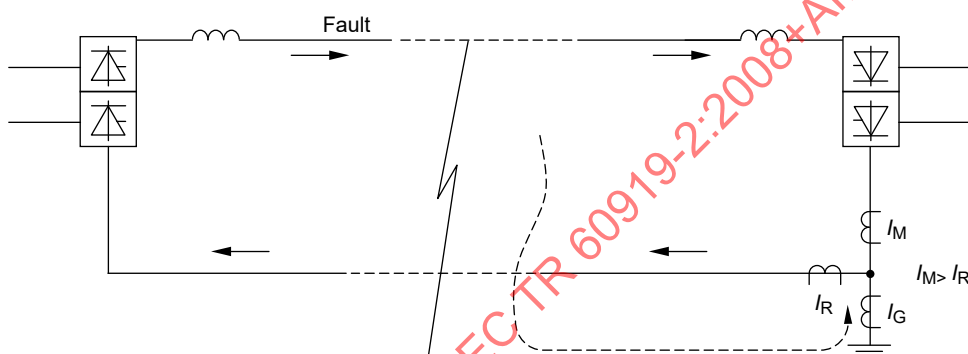
Figure 15a – Metallic return conductor fault to earth
