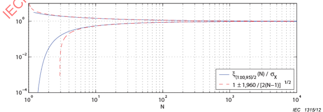
Figure 13 – 95 % confidence intervals for S_X as a function of N for measurements using a single-axis detector
