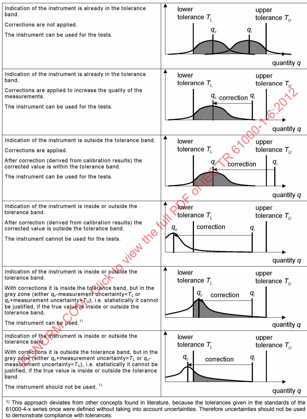
Figure 17 – Situations, where and how an instrument is suitable for tests and/or measurements as specified in the applicable basic standard with tolerances
