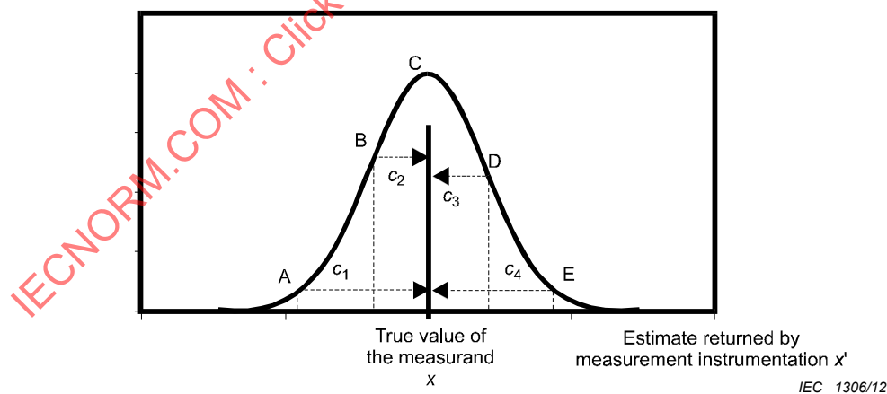
Figure 4 – Impact of g(x) on interpretation of x'
