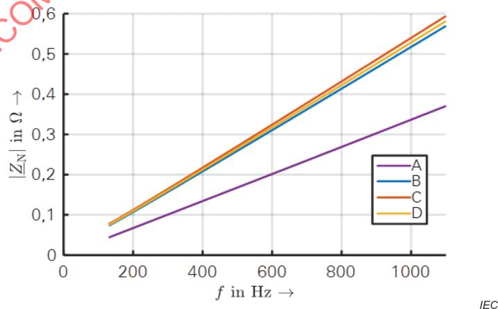
Figure 18 – Simulated network harmonic impedance at different locations (L1-N) using default element representations
