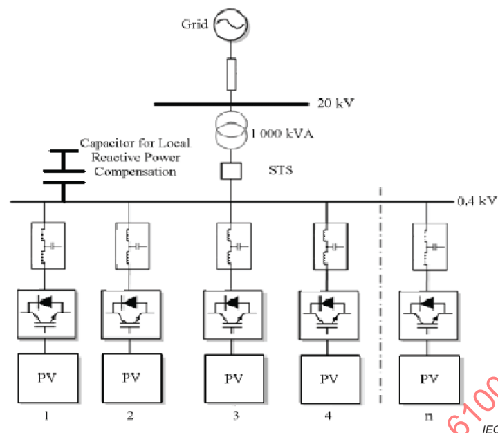
Figure 50 – Parallel-connect configuration in large photovoltaic (PV) farm
