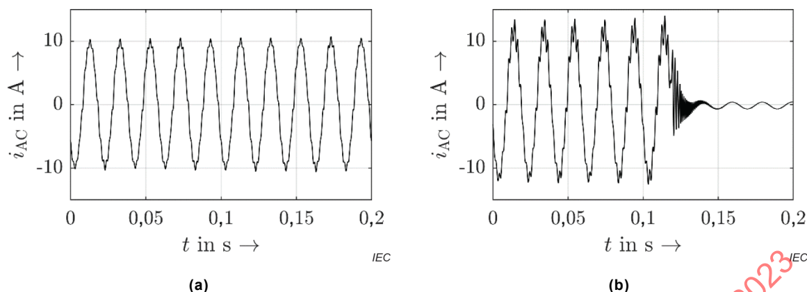
Figure 80 – Grid-side current measurements for LR -equivalent network impedance with inductance values of 2,3 mH (a) and 3,2 mH (b)
