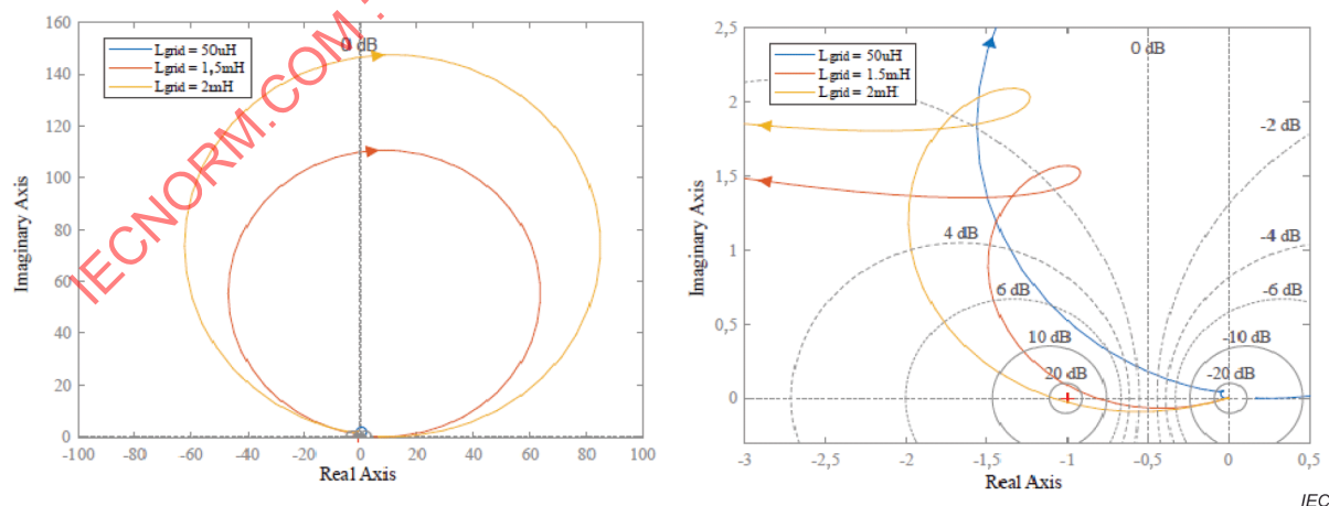
Figure 75 – Nyquist stability analysis of the control loop with parameters listed in Table 8
