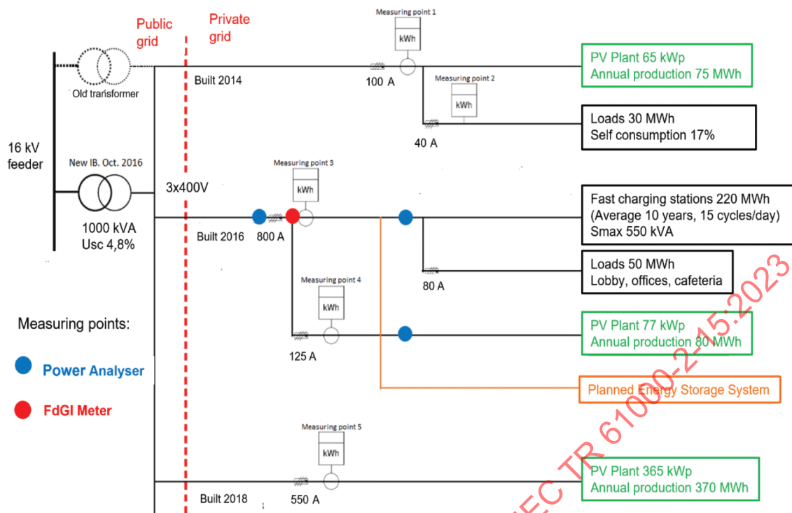
Figure 11 – Bloc scheme of the measured EV charging hub with PV production
