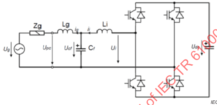
Figure 71 – Single phase inverter with an LCL filter and corresponding state variables
