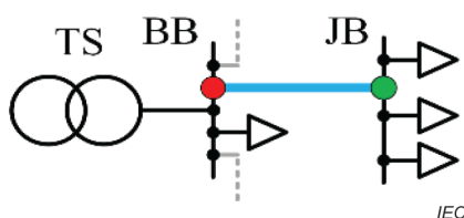
Figure 31 – Single-line diagram of relevant parts of the low voltage network
