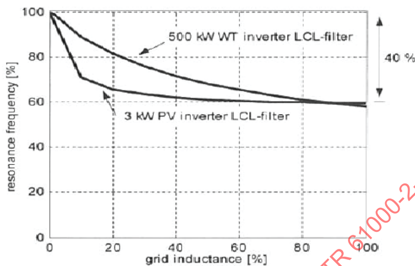
Figure 100 – Resonance frequency variation in per cent of the rated resonance frequency as a function of grid inductance in per cent
