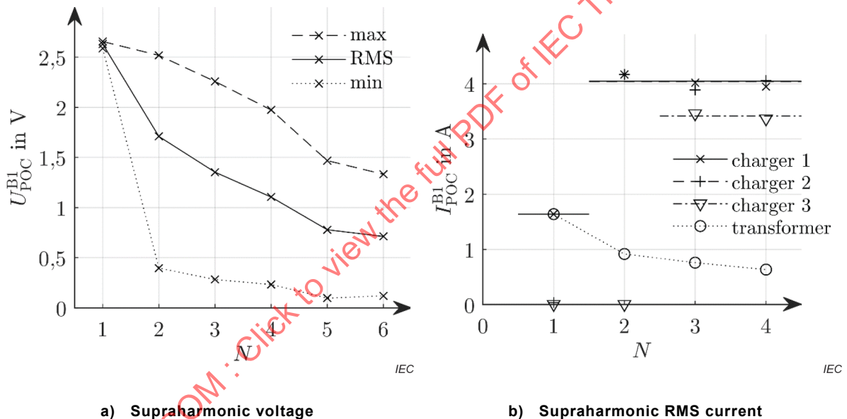
Figure 65 – Supraharmonic voltages and currents at the POC of multiple AC charging points, first emission band (800 Hz) centred around 10 kHz
