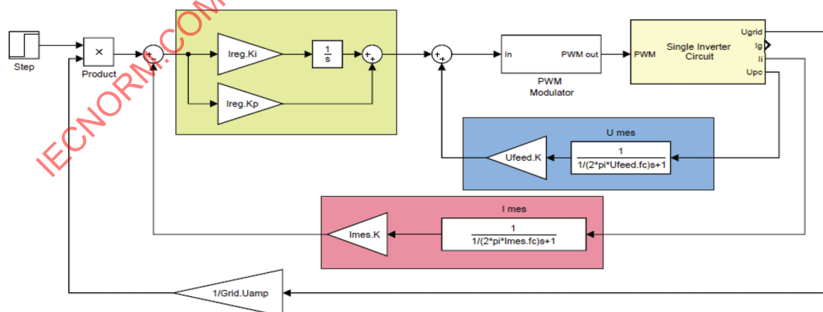
Figure 77 – PLECS model of the single-phase inverter controller with Feedforward of the connecting point voltage
