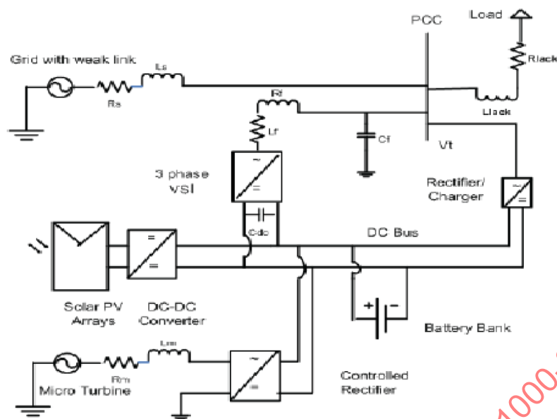
Figure 95 – Description of the circuit including a solar PV–micro turbine based power system with battery backup
