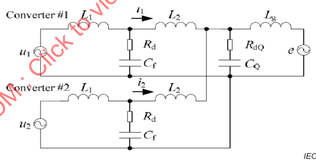
Figure 51 – Simplified parallel of two converters featuring LCL filter and capacitor on common bus for reactive compensation in the grid (see Table 7)
