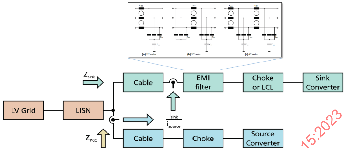
Figure 60 – Modeling of a simple configuration of noise source and noise sink, where the EMI filter of the sink converter can be of 2 nd , 3 rd or 4 th order [25]
