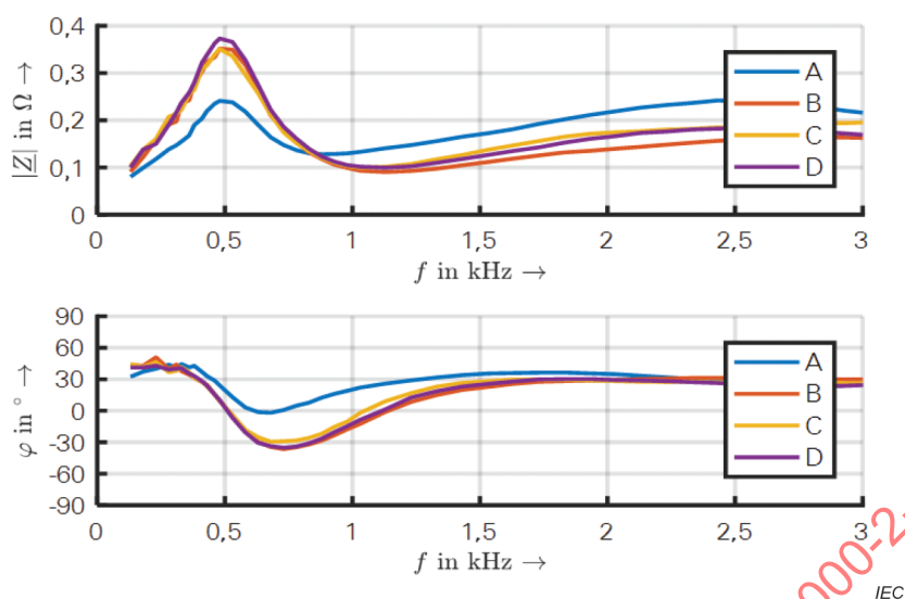
Figure 17 – Network harmonic impedance measured at different locations (L1-N)
