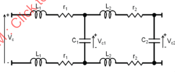
Figure 88 – Description of the low frequency filter
