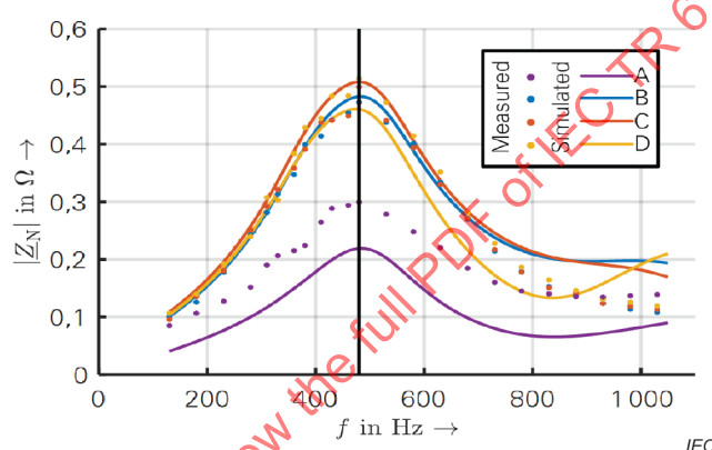
Figure 20 – Measured and simulated network harmonic impedance at different locations (L1-N) using the developed customer impedance model
