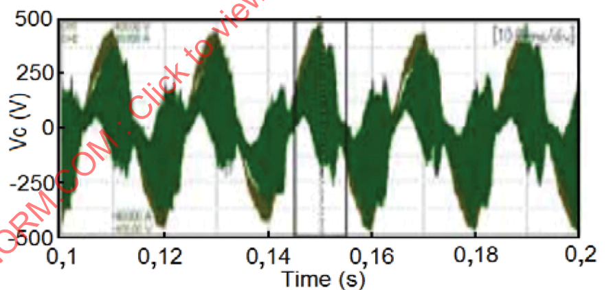
Figure 94 – Voltage V_{cmeas} at the entrance of the charger, measured at the manufacturer's laboratory, for a value of 750 \mu H for the inductance of the upstream network
