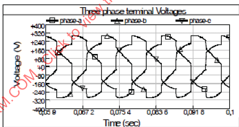
Figure 96 – PCC (grid) voltage with linear and non-linear loads in the absence of any VSI (voltage source inverter)
