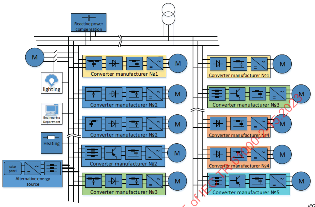
Figure 58 – Configuration of an industrial grid
