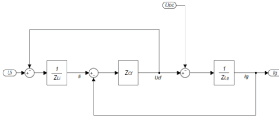
Figure 72 – Block scheme equivalent to the formula system of Figure 71
