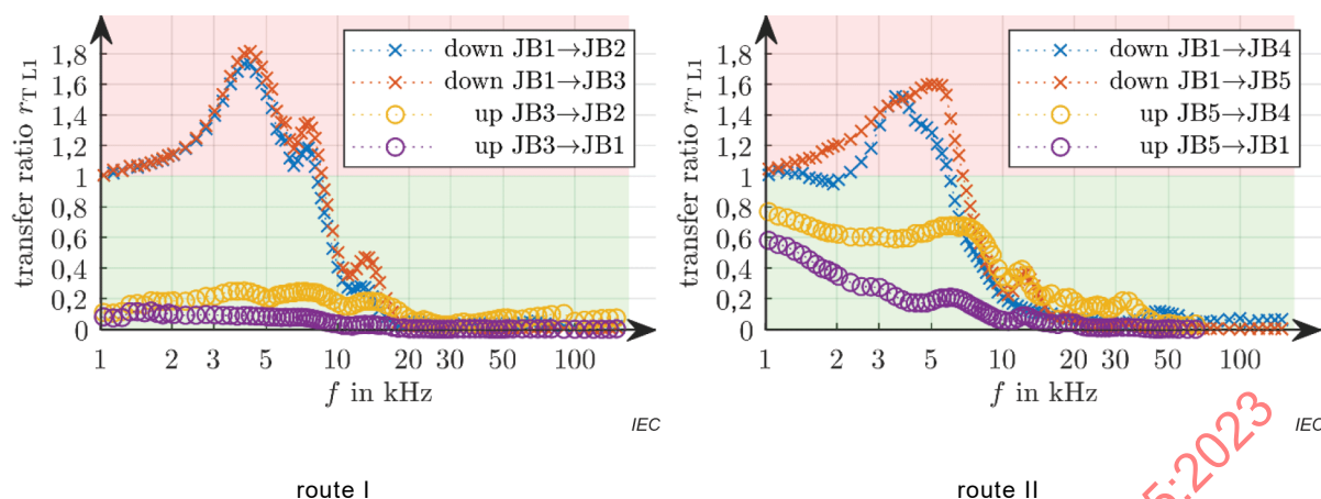
Figure 41 – Transfer ratios along two routes in a low voltage network with residential customers, upstream direction as circles, downstream direction as crosses
