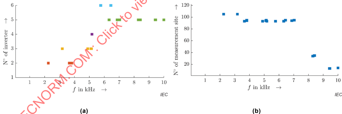
Figure 84 – Critical frequency regions of commercially available inverters (a) and measurement sites in LV networks (b)
