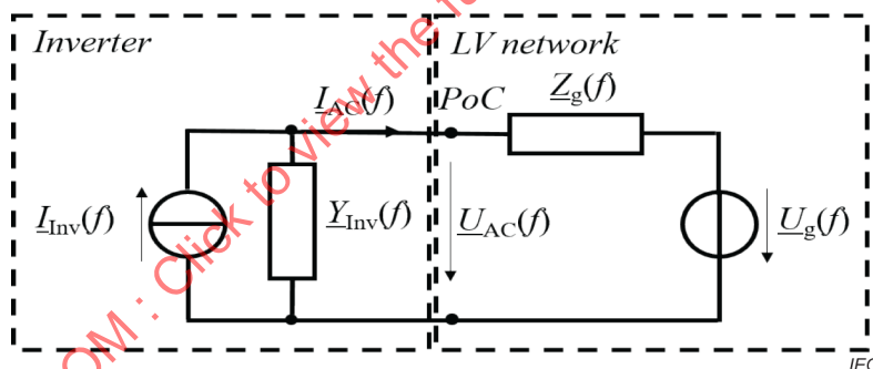
Figure 81 – Small signal model of an inverter and the low voltage network
