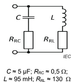
Figure 19 – Equivalent impedance model of a domestic customer
