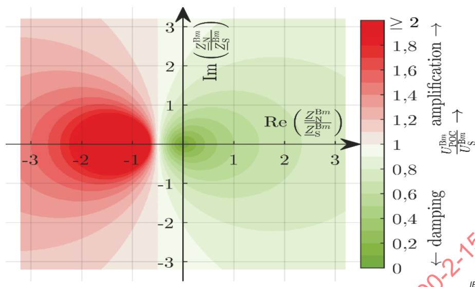
Figure 44 – Amplification and damping of supraharmonic emission at the POC relatively to the source voltage depending on the network to source impedance
