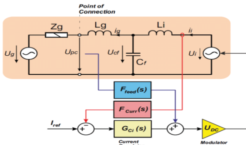
Figure 73 – Linearized control loop for the in-feed converter and transfer functions for feed forward and current measurement filter
