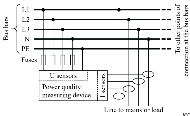
Figure 25 – Connection of a PQ measuring device
