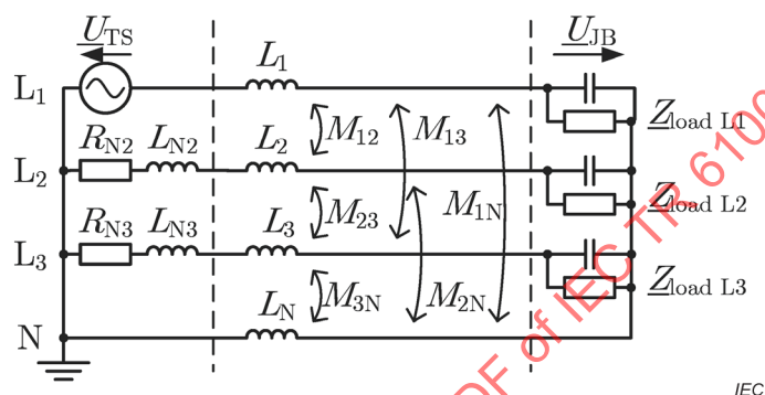
Figure 37 – Simplified simulation model for supraharmonic transmission along a low voltage cable
