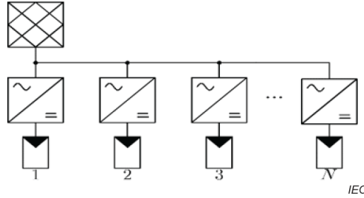
Figure 66 – Single-line diagram of an arbitrary number N of power converters operating in parallel on a single network phase
