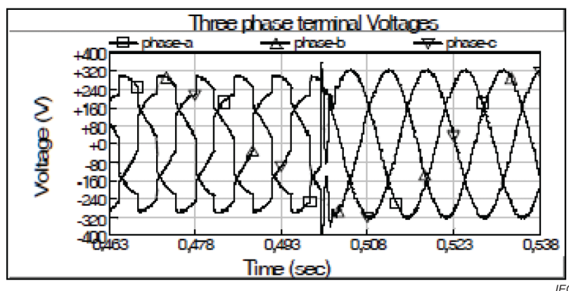
Figure 97 – Grid working and VSI switched on at t = 0,5 s
