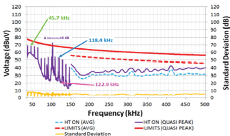
Figure 49 – Identification of the frequencies in the spectrogram of the measurements (see case study [23])
