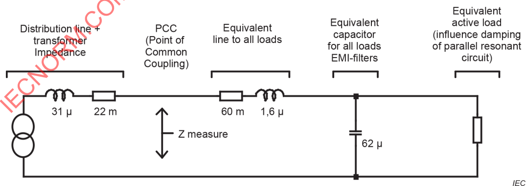
Figure 13 – Resulting simplified model of the charging hub with distribution lines and feeder
