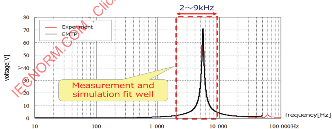
Figure 7 – Resonance magnification factors (RMFs) using measurement and simulation
