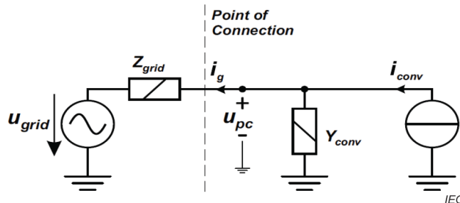
Figure 74 – Norton equivalent circuit of the single-phase inverter
