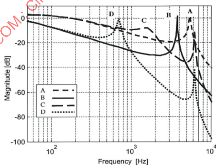
Figure 99 – Frequency characteristic of the 3 kW PV system with L-C-L filter in the following grid conditions: A) 0,1 mH, B) 3 mH, C) 0,1 mH, 100 \mu F and D) 3 mH, 100 \mu F
