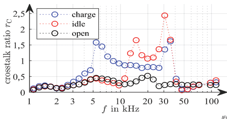
Figure 33 – Crosstalk ratio of supraharmonic voltage between phase L1 (phase of injection) and phase L2 at the junction box JB
