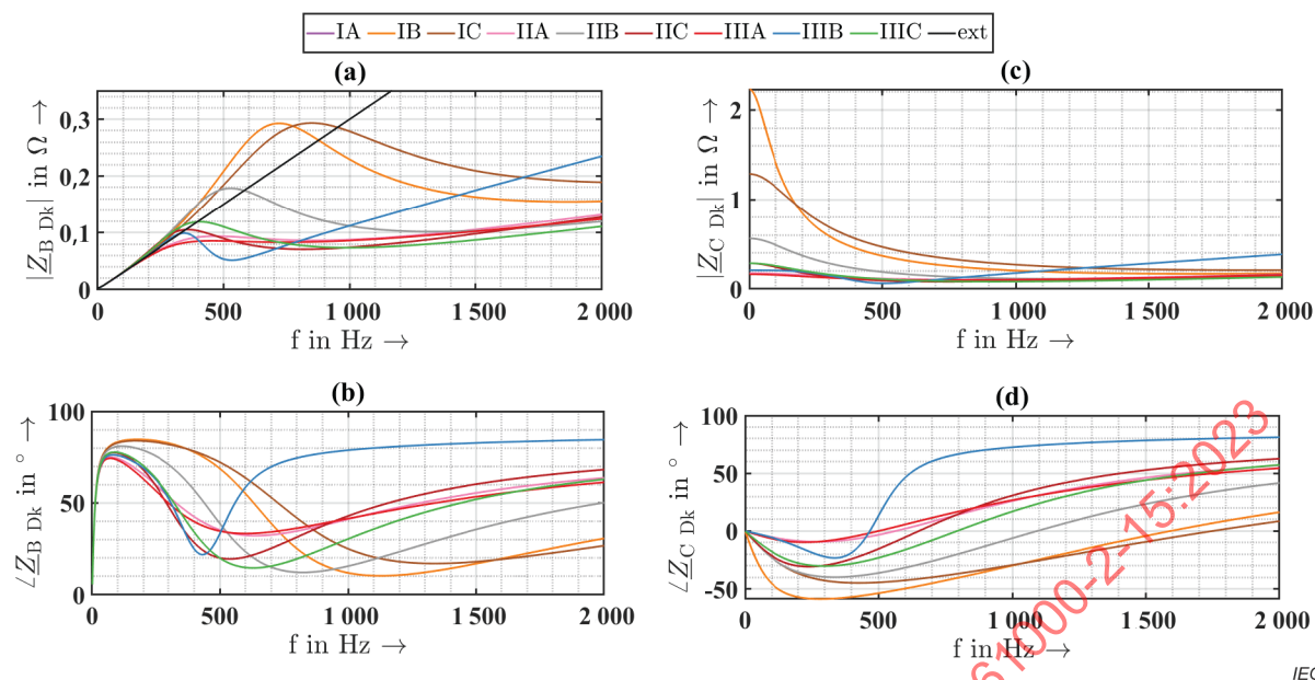
Figure 15 – Impedance characteristics of an urban LV network,
