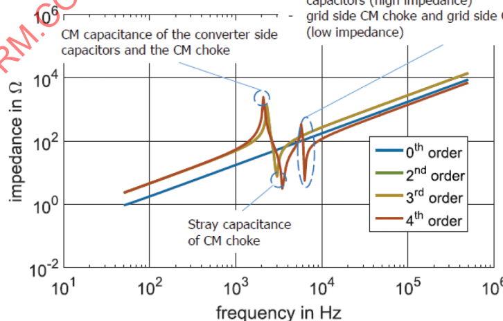
Figure 61 – Impedance into the noise sink converter Z_{\text{sink}} with different EMI filter types with simple choke interface only and different EMI filter configurations
