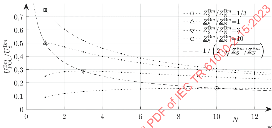
Figure 70 – Dependency of the POC voltage on the number of sources N for different magnitude ratios of source impedance to network impedance assuming phase angles of source impedance and network impedance are equal
