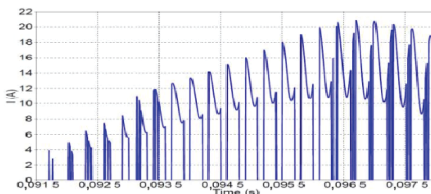
Figure 93 – Current crossing an IGBT obtained by simulations, with an inductance value of 600 \mu H for the upstream network
