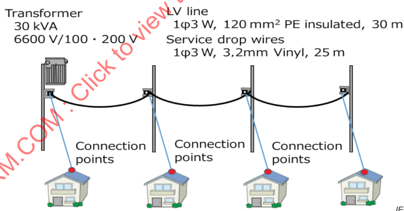
Figure 5 – Description of the experimental test configuration
