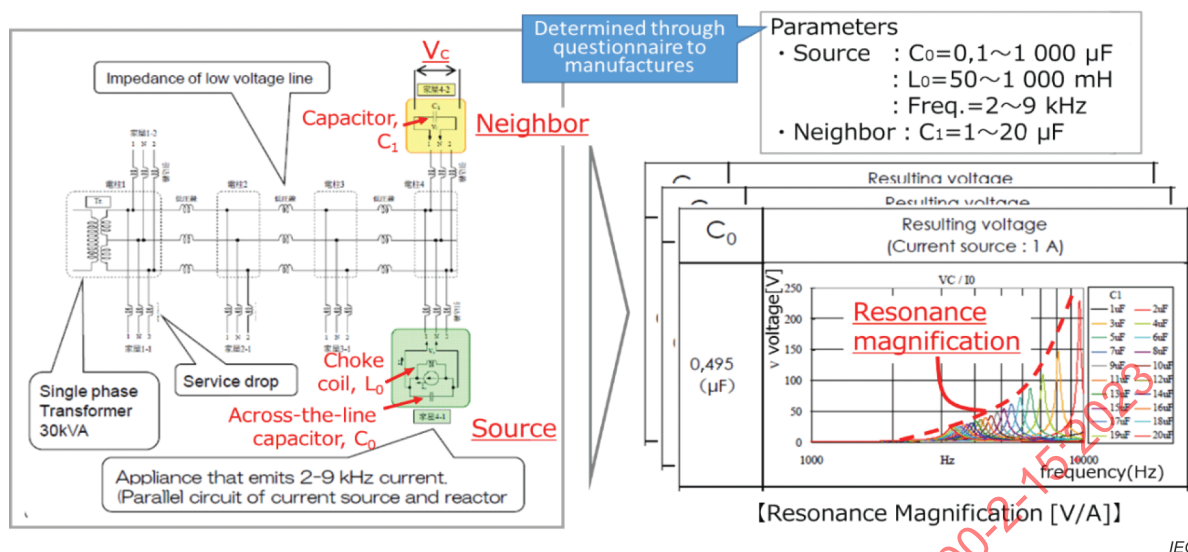
Figure 4 – Electrical circuit used in simulations, and results of resonance magnification factors (RMFs)
