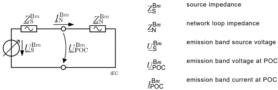
Figure 42 – Equivalent circuit (model) for the supraharmonic emission of single-phase voltage-source power converters for the m^{\text{th}} emission band
