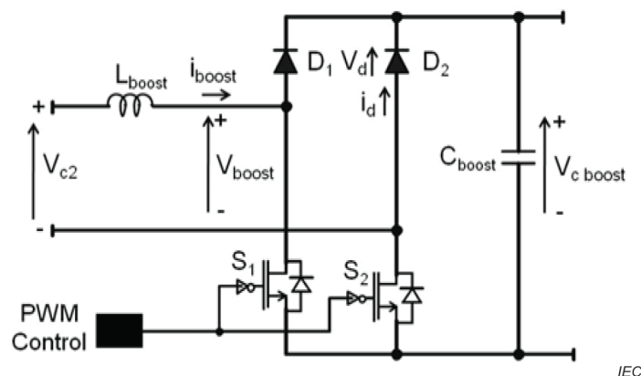
Figure 89 – Description of the converter of the boost PFC converter, including its AC/DC rectifier
