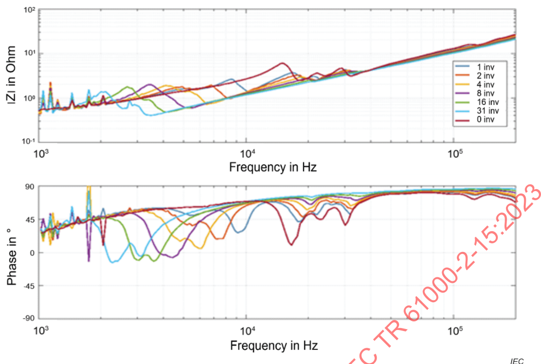
Figure 57 – Power line impedance measured with 0 to 59 inverters activated in a 2,1 MW PV plant
