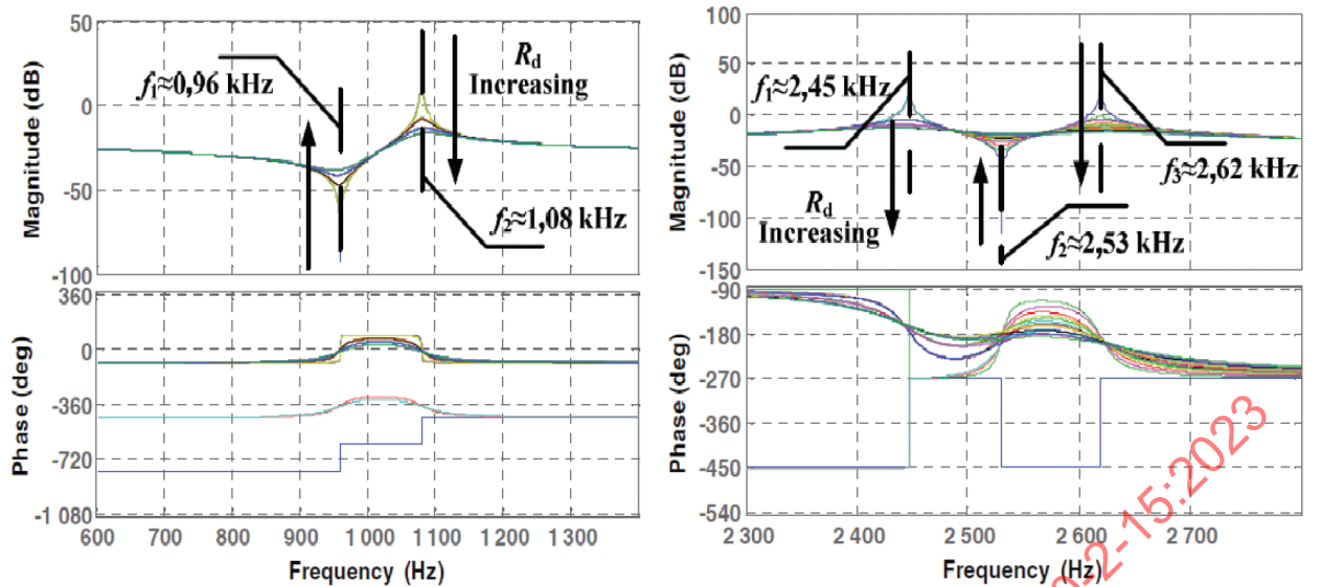
Figure 52 – Frequency domain results of parallel LCL filter system with reactive power compensation capacitor represented in two frequency ranges
