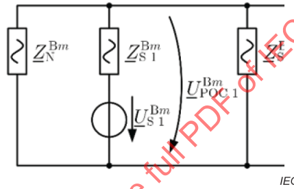
Figure 67 – Supraharmonic emission model for an arbitrary number N of power converters operating in parallel
