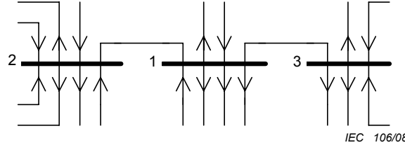
Figure 7 – Determination of S_t for a meshed HV or EHV system
