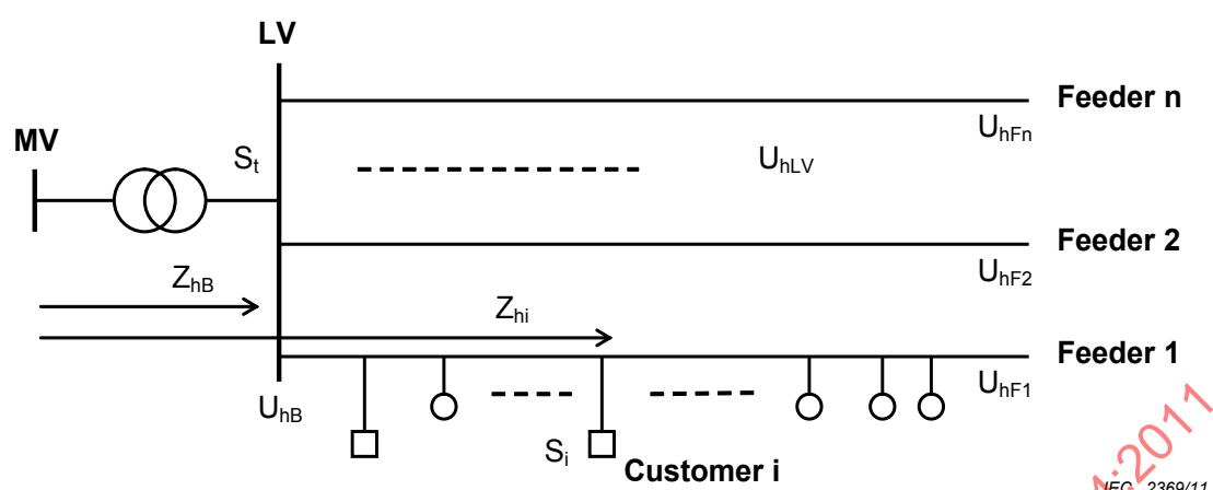
Figure C.1 – Scheme of an LV public system
