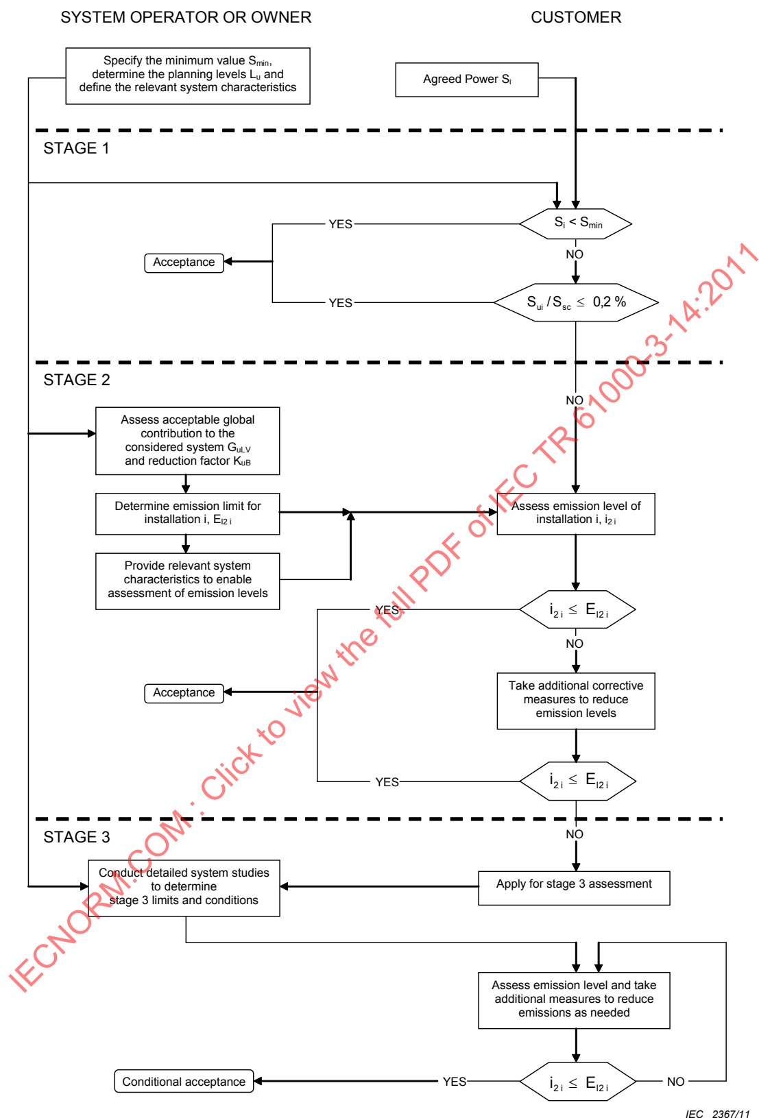
Figure 10 – Diagram of evaluation procedure for unbalance
