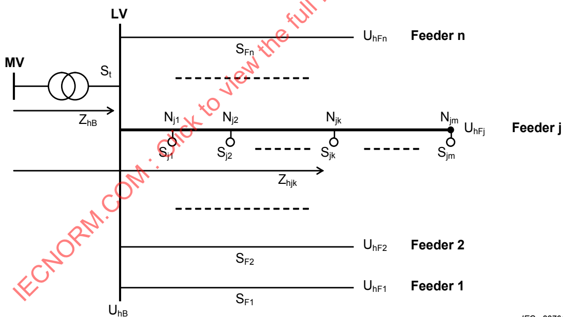
Figure D.4 – Simplified scheme of an LV public system for the calculation of harmonic voltage levels at the far end of LV feeders
