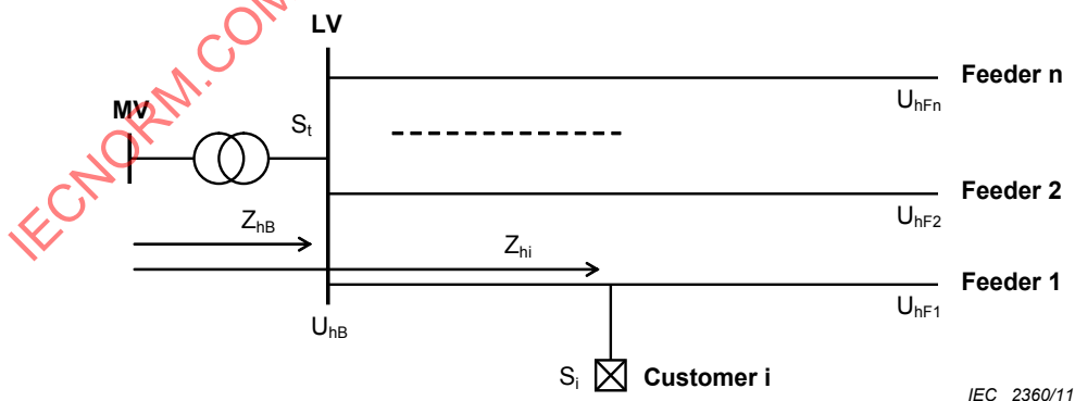
Figure 4 – Simplified scheme of an LV public system for harmonics
