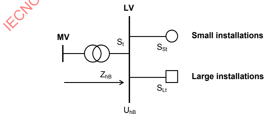
Figure C.3 – Simplified scheme of an LV public system in order to work out the condition at the LV busbar
