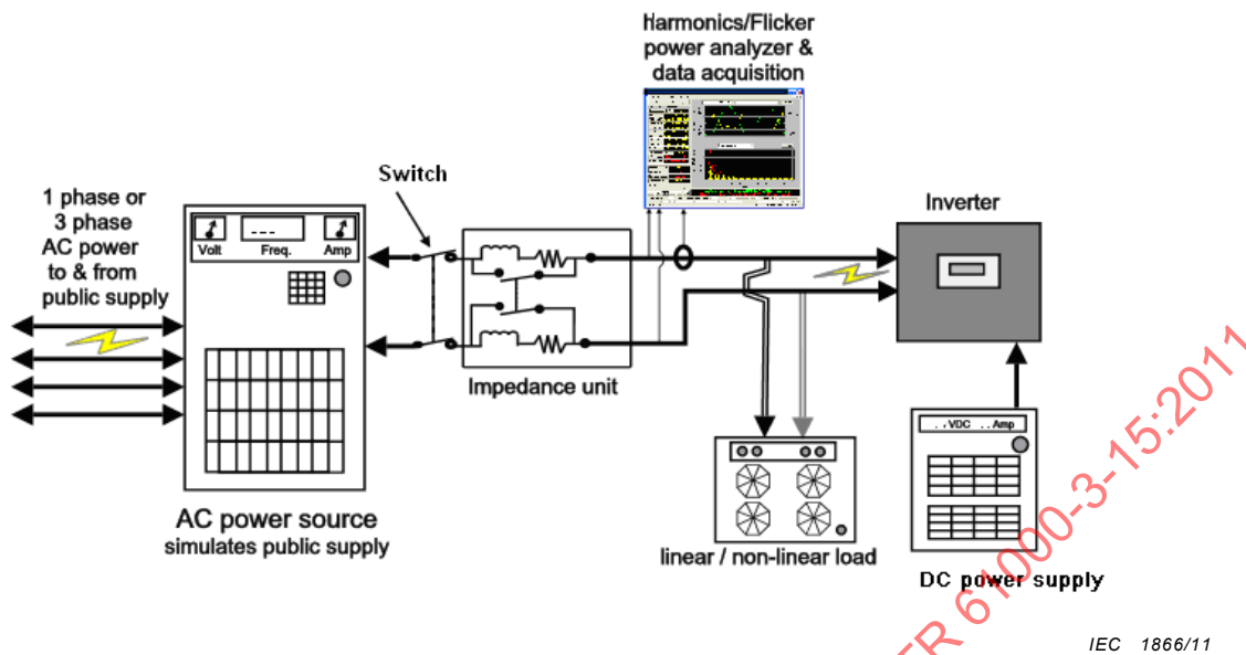
Figure 1 – General test setup for combined emission/immunity tests
