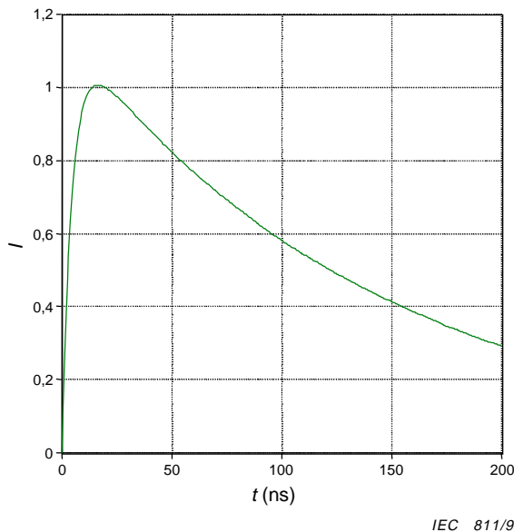
Figure A.3a – Time-domain behaviour
