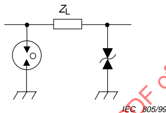
Figure 4 – Circuit de protection type
