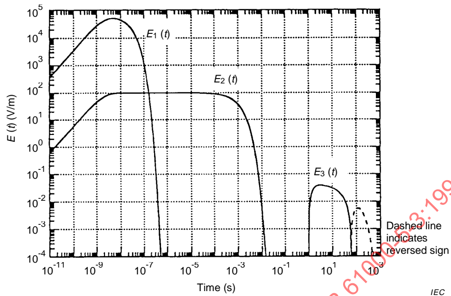
Figure A.1a – Time domain behaviour
