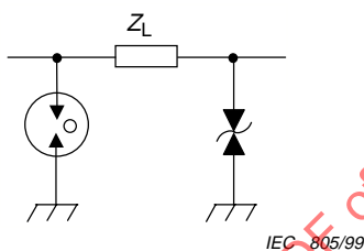
Figure 4 – Typical protection circuit
