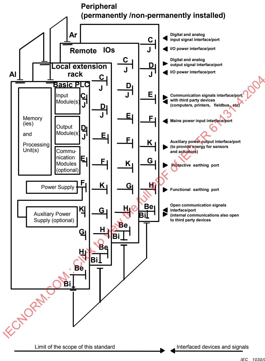
Figure A.3 – Typical interface/port diagram of a PLC system
