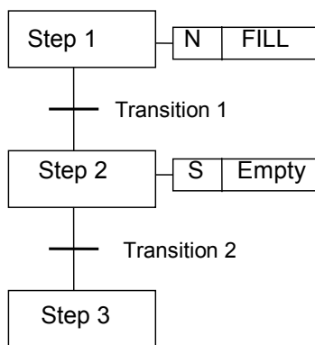
Figure A.12 – Sequential function chart
