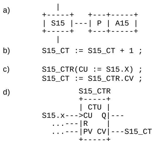
Figure 18 – Use of pulse (P) qualifier a) SFC fragment b) Incorrect body for action A15 (ST language) c) Correct body for action A15 (ST language) d) Correct body for action A15 (FBD language)
