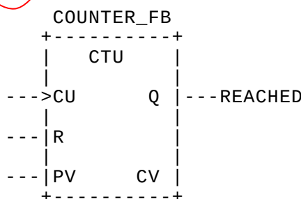
Figure 12b – Graphical invocation
