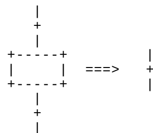
Figure 28b – A sequence consisting of a transition, a step and a transition is replaced by one transition
