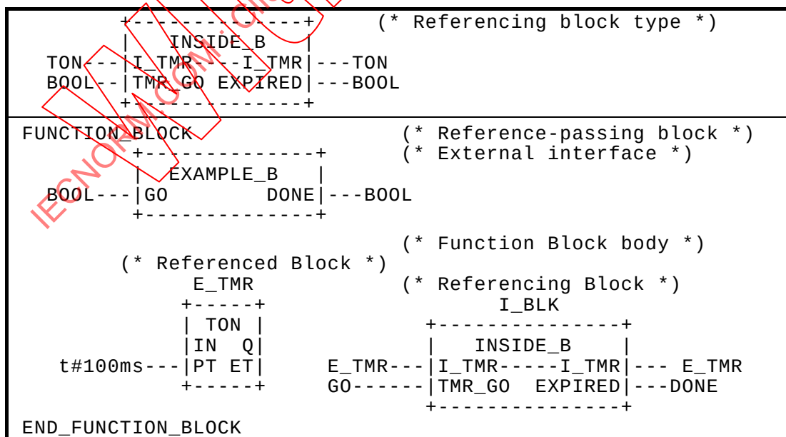
Figure 10b – Function block name used as an in-out variable
