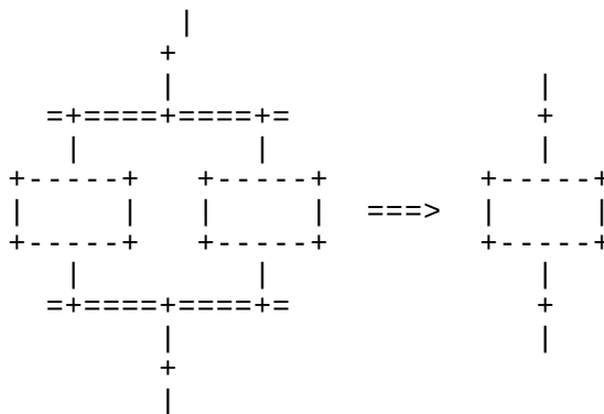
Figure 28d – A simultaneous sequence (AND branch) is replaced by one step
