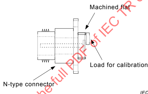
Figure 16 – Possible solution for calibration of reference loads
