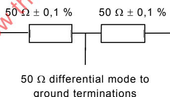
Figure 17 – Resistor termination networks
