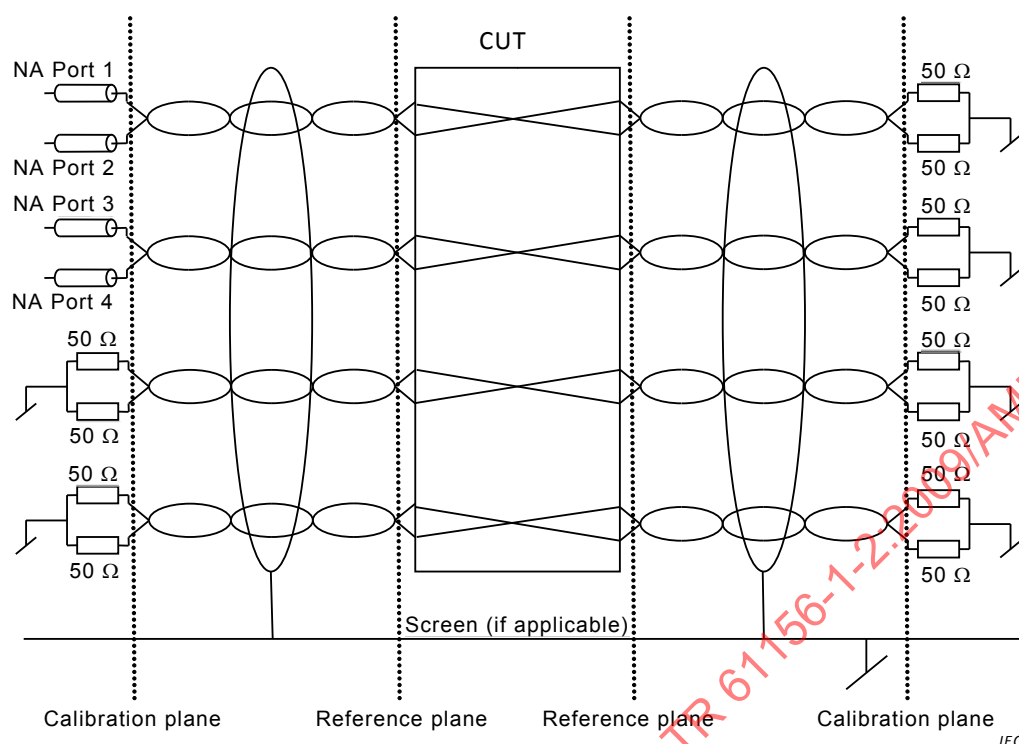
Figure 19 – NEXT measurement
