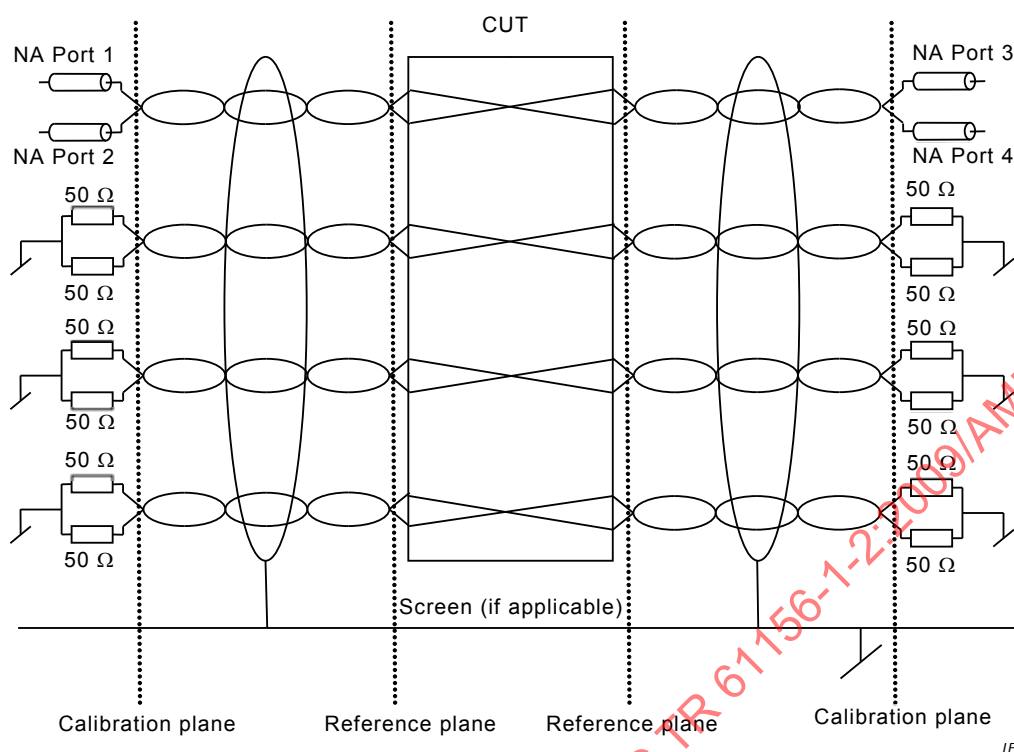
Figure 18 – Insertion loss and EL TCTL measurement
