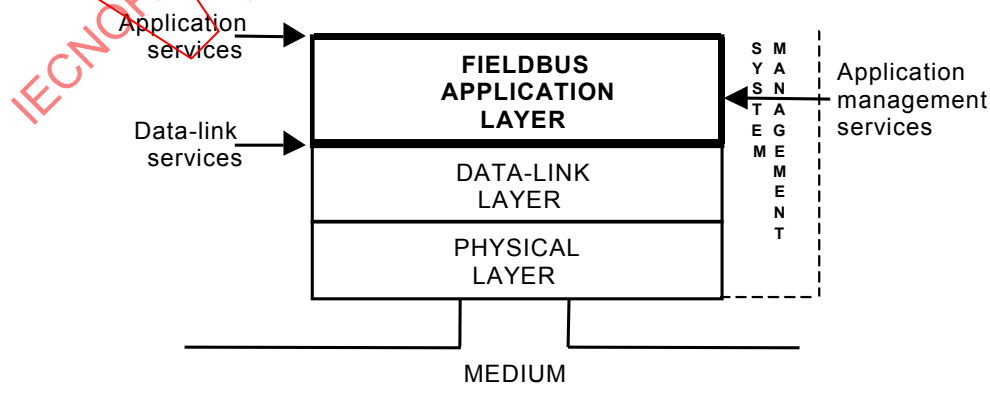
Figure 6 – Relationship of the IEC 61158-5 and IEC 61158-6 series to other fieldbus layers and to users of the fieldbus application service
