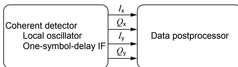
Figure 4 – Block diagram of the main functions for vector signal measurement
