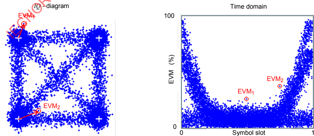
Figure 15 – IQ-diagram with indicated reference constellation and exemplary error vectors (left) and time domain plot of the EVM values for each measured sample (right)
