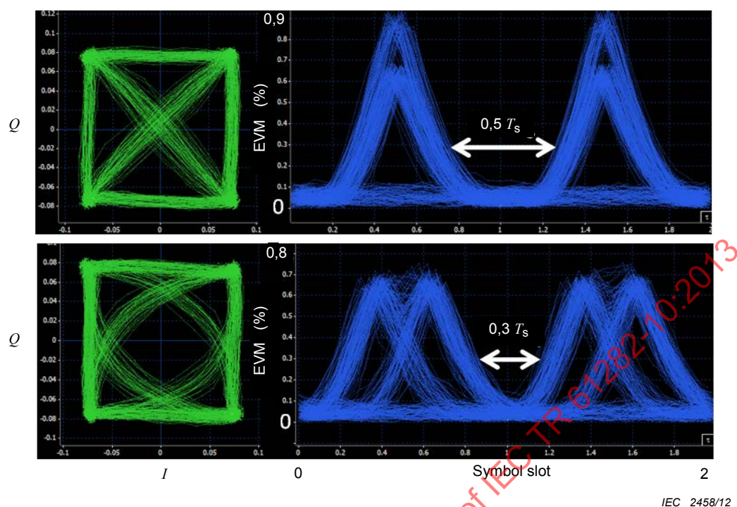
Figure 17 – Noise-averaged IQ-diagrams and time-resolved EVM plots of a 28 GBd QPSK signal with 0 p skew (top) and 8 ps skew (bottom)
