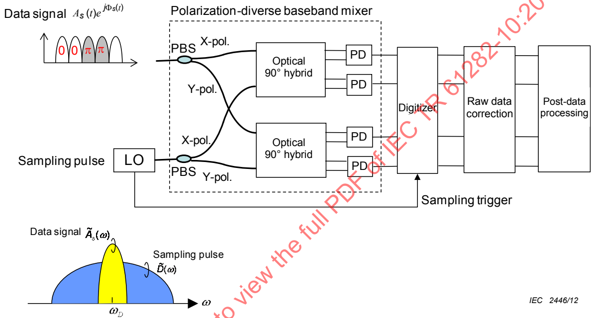
Figure 6 – Configuration for linear optical sampling
