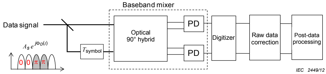
Figure 8 – One-symbol delayed interferometer for detecting differential phase modulation
