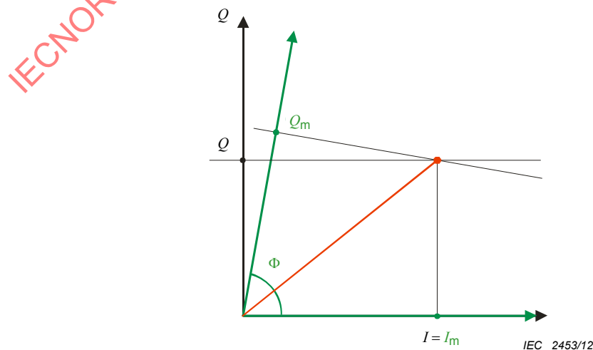
Figure 12 – Error in I and Q determination from phase angle deviation
