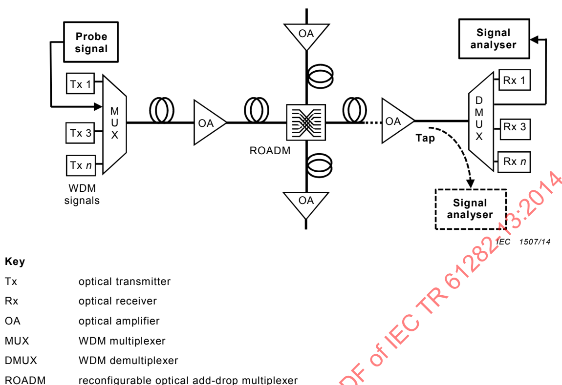
Figure 3 – Semi-intrusive in-service fibre characterization using narrowband probe signal
