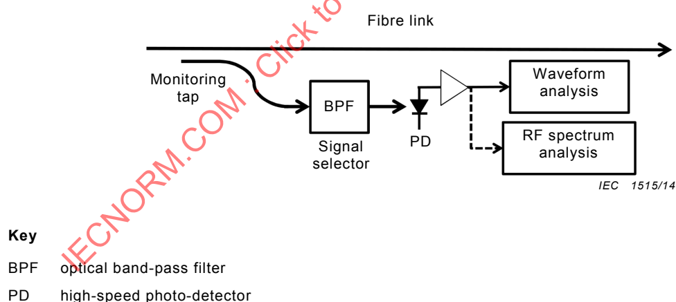
Figure 11 – Apparatus for GVD measurements in a transmitted signal using a high-speed receiver with time-domain waveform analysis or, alternatively, RF spectrum analysis
