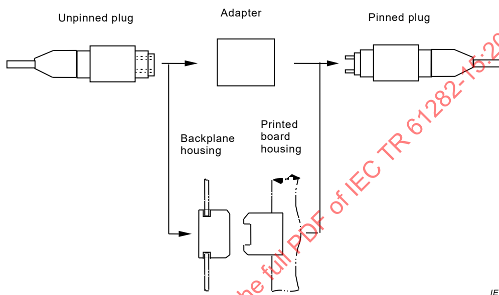
Figure 1 – MPO connector
