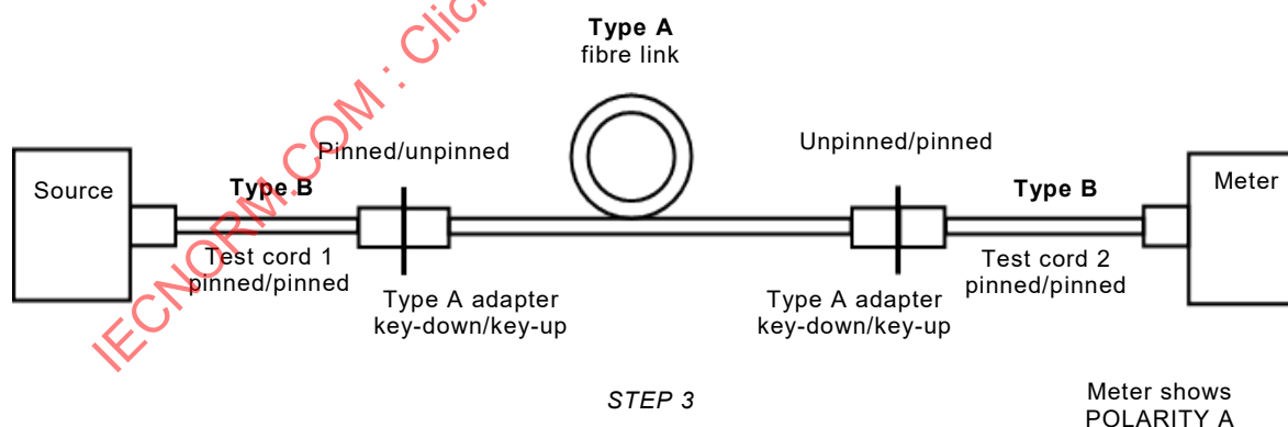
Figure 4 – Reference connections for cabling with unpinned MPO plugs
