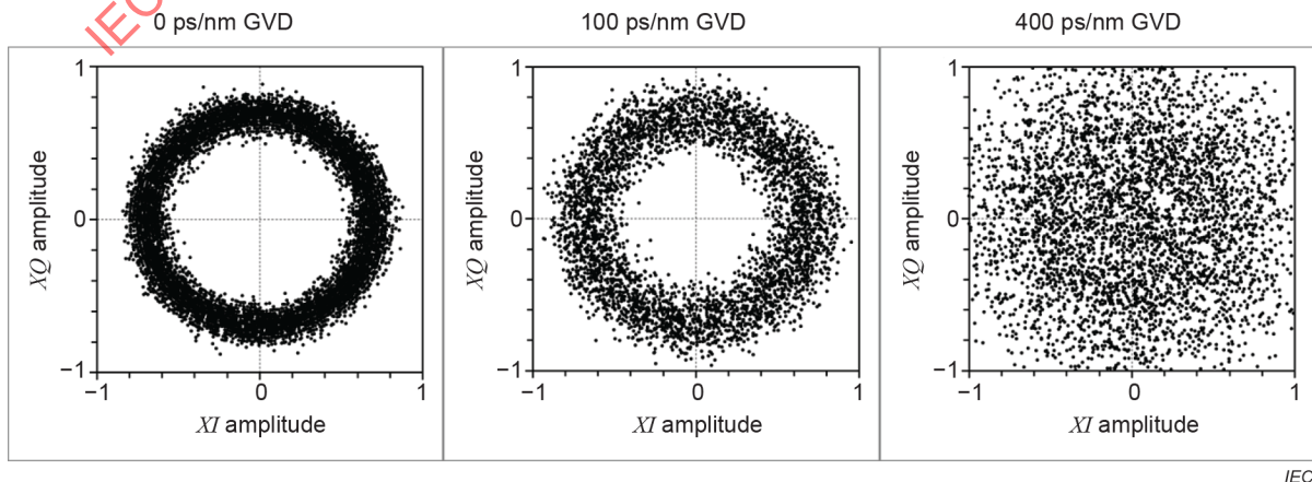
Figure 32 – QPSK signal constellations for various amounts of GVD
