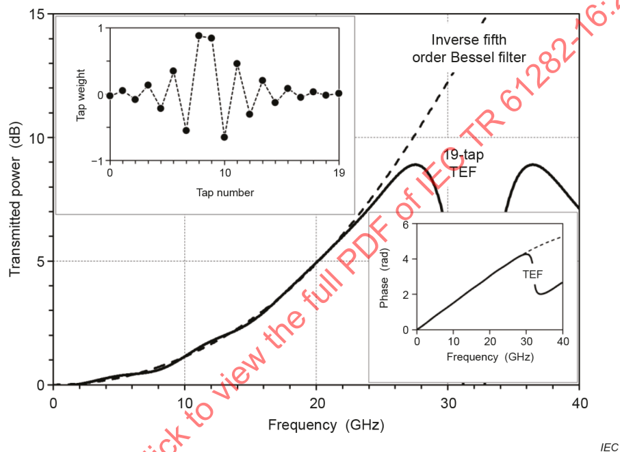
Figure 23 – Amplitude and phase of FSE-generated inverse Bessel filter
