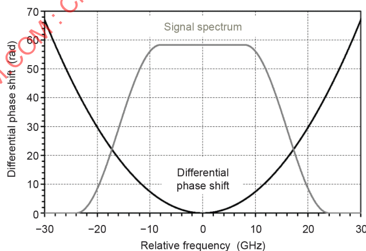
Figure 12 – Differential phase shifts introduced by 3 000 ps/nm GVD
