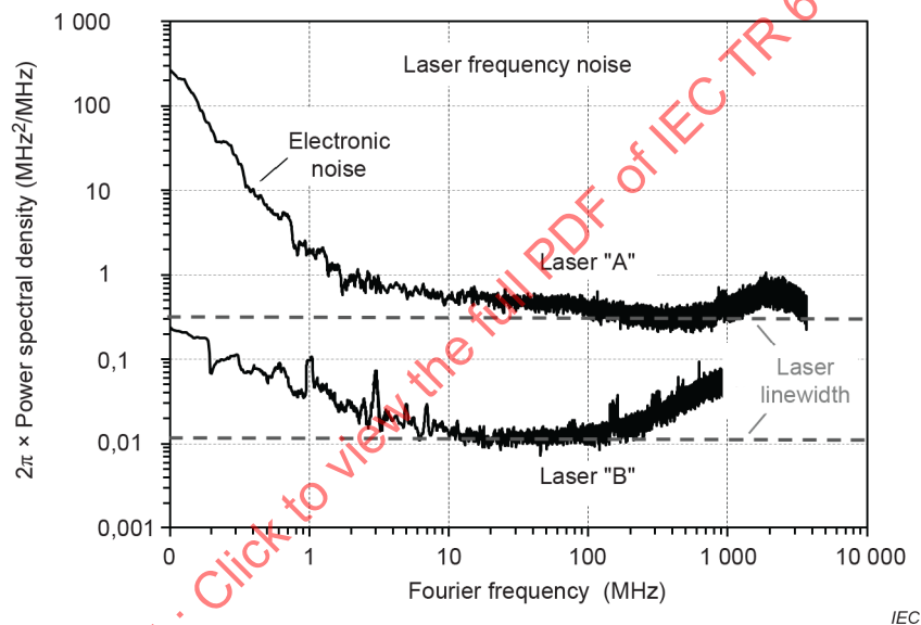
Figure 34 – Optical frequency noise spectra of two lasers
