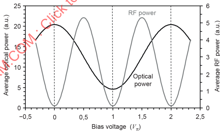
Figure 52 – Optical and RF output power versus bias voltage for linear operation
