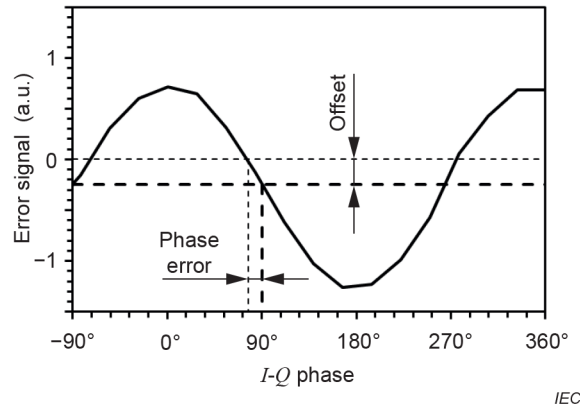
Figure 56 – I-Q phase error resulting from offset in feedback signal
