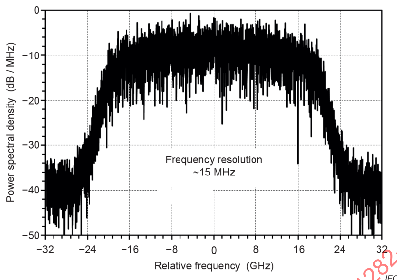
Figure 38 – High-resolution optical spectrum of a 32 GBd QPSK signal
