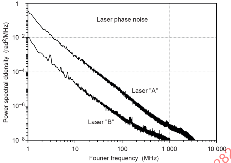
Figure 35 – Optical phase noise spectra of two lasers
