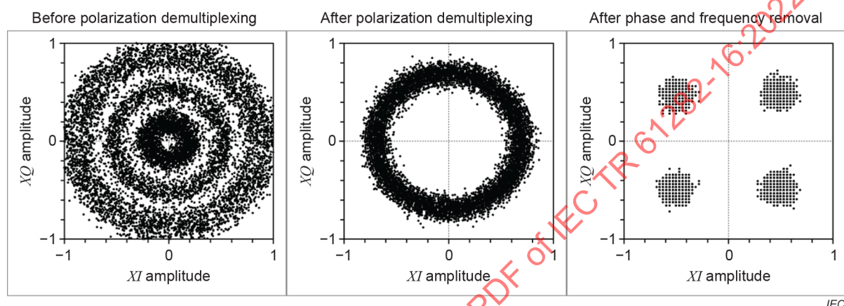
Figure 27 – Constellation points of QPSK signal after polarization demultiplexing
