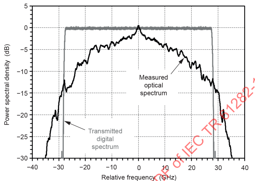
Figure 61 – Magnitude of transmitter frequency response
