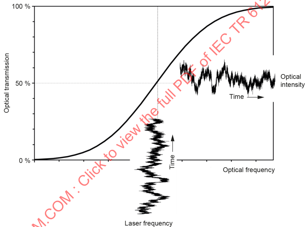
Figure 36 – Laser phase noise measurement with optical bandpass filter
