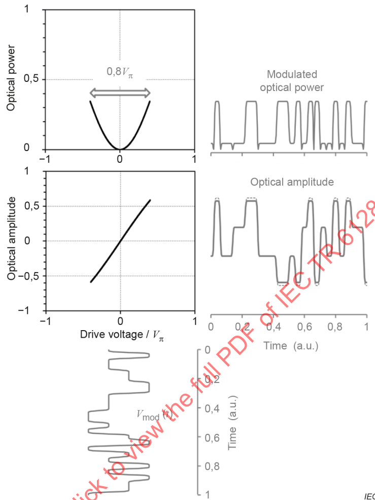
Figure 50 – Linear MZM operation for quaternary ASK signals
