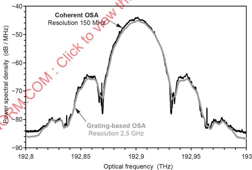
Figure 39 – QPSK signal measured with coherent OSA and with grating-based OSA
