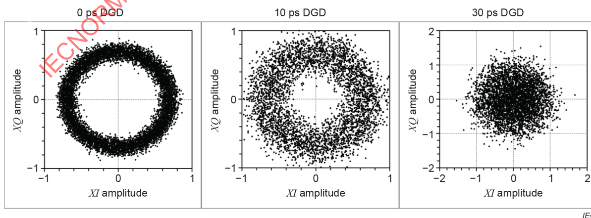
Figure 30 – QPSK signal constellations for various amounts of PMD
