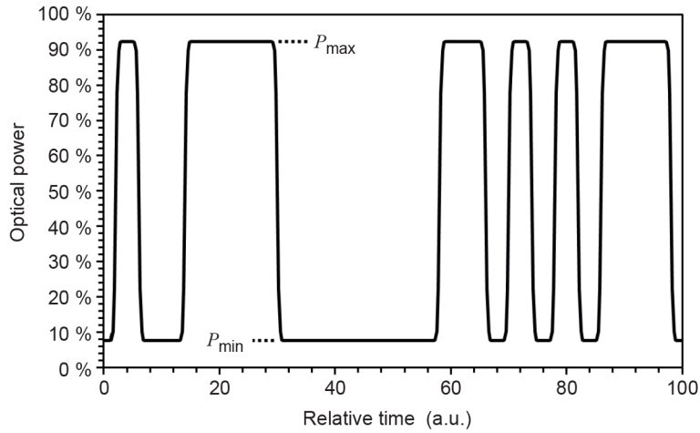
Figure 51 – Optical power variations in an NRZ-OOK signal with finite extinction ratio
