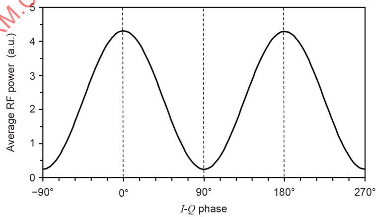
Figure 54 – RF output power of I - Q modulator versus I - Q phase
