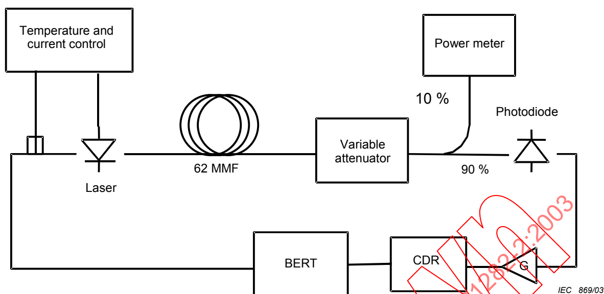
Figure 3 – Experimental set-up for link measurements
