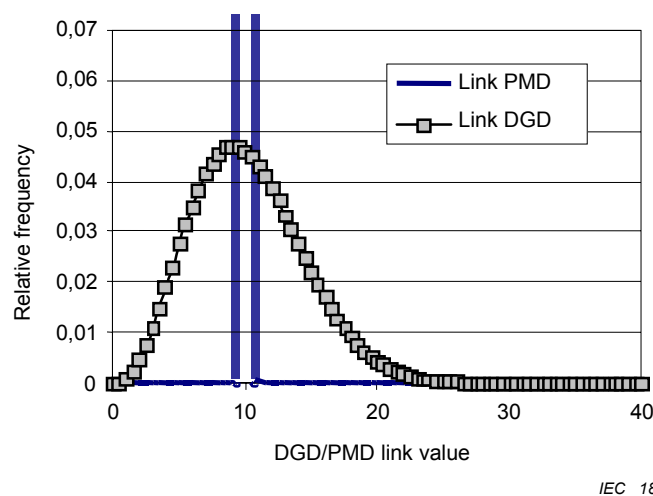
Figure 2 – Worst case approach assumption
