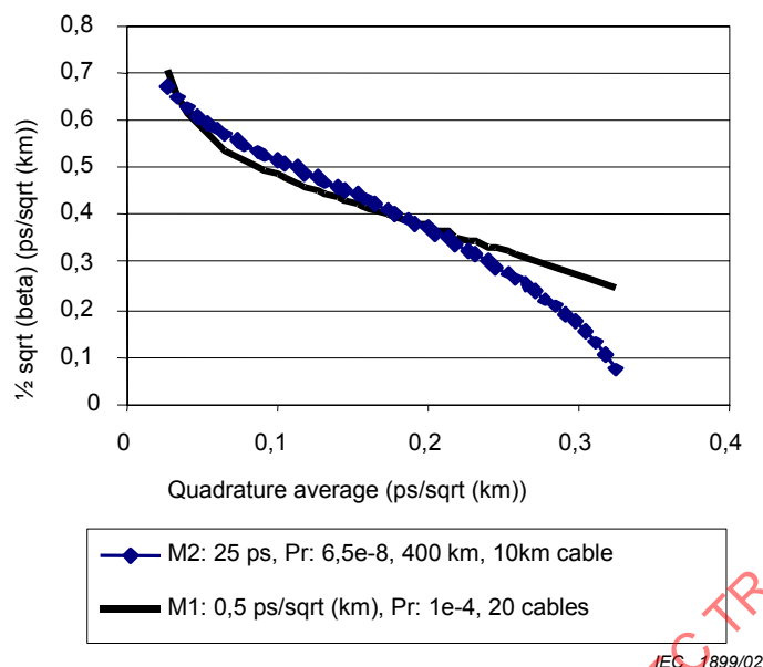
Figure 4 – Equivalence envelopes for method 1/2 defaults
