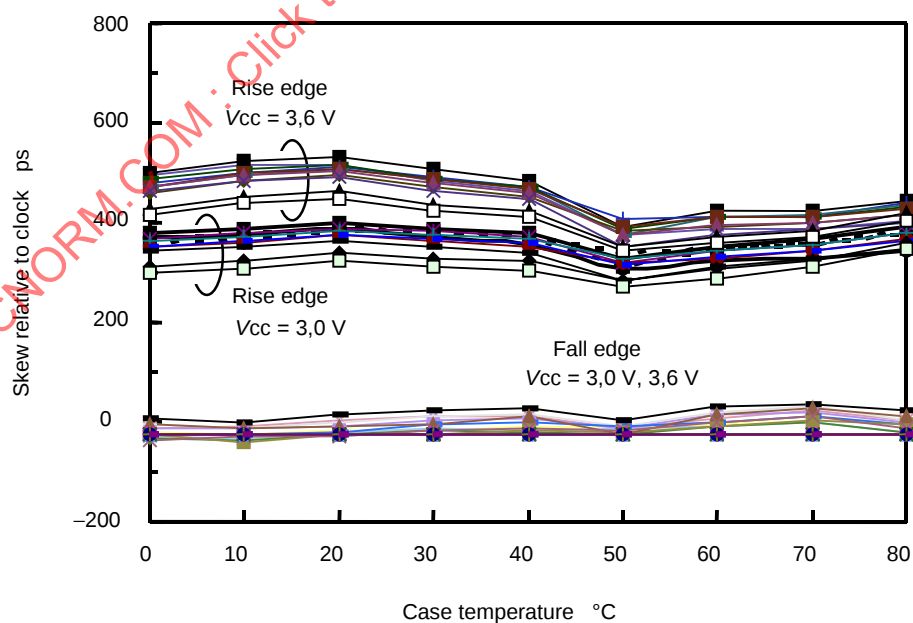
Figure 14 – Temperature dependence of transmitter skew
