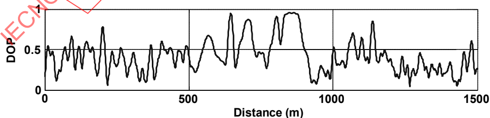
Figure 34 – Degree of polarization (DOP) vs. distance for a concatenation of three 500-m fibres, with a centre fibre that exhibits a high h value
