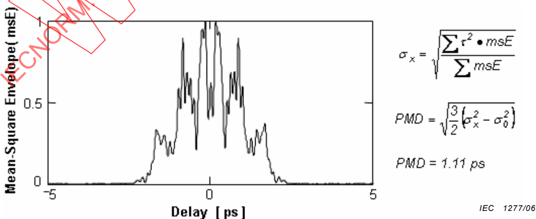
b) PMD obtained from GINTY analysis with the mean-square envelopes
