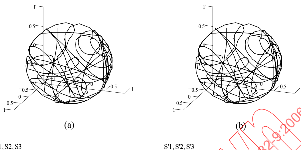
Figure 15 – Trajectories of the principal states of polarization on the Poincaré sphere from a) Jones matrix eigenanalysis (JME) and b) Poincaré sphere analysis (PSA)
