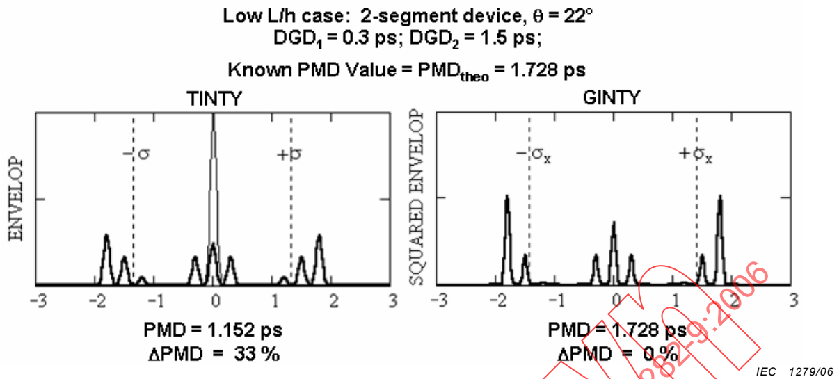
Figure 28 – Comparison between polarization mode dispersion results from TINTY and GINTY analyses
