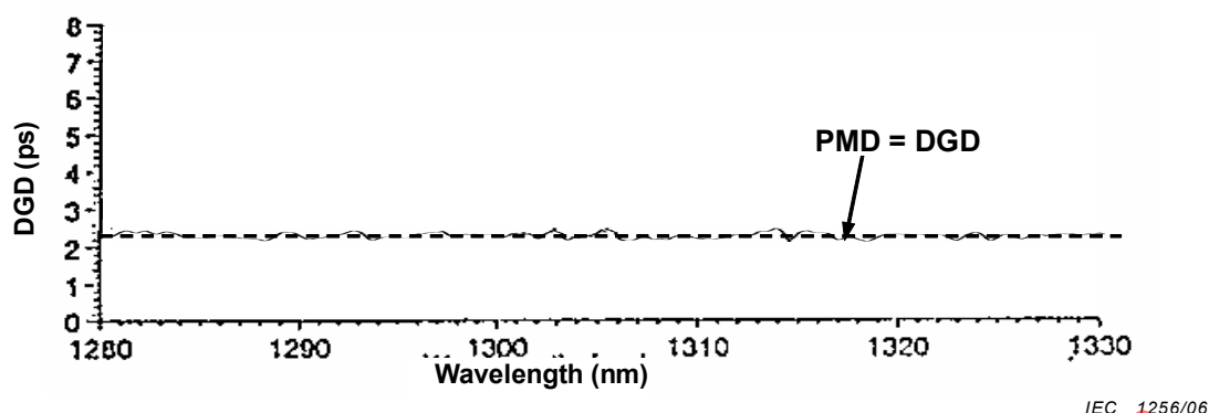
Figure 9 – Polarization mode dispersion and differential group delay in negligible mode coupling
