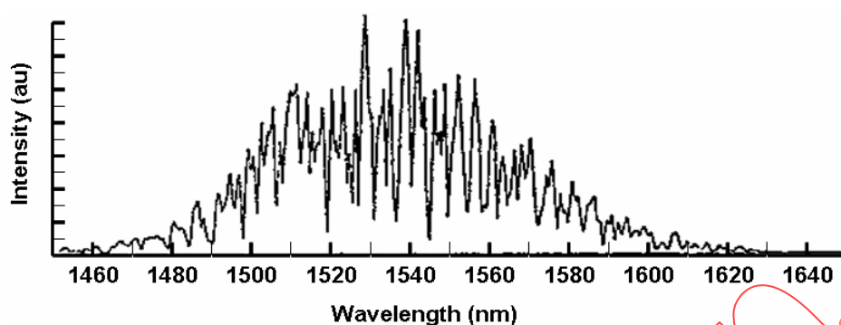
a) Spectral intensity
