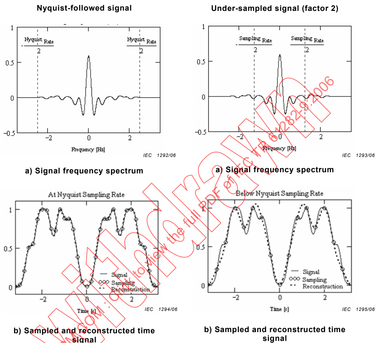
Figure 39 – Filtered signal with Nyquist-based defined bandwidth
