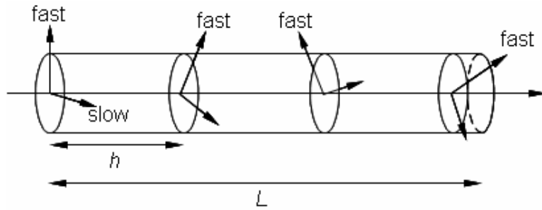
Figure 7 – Random mode coupling
