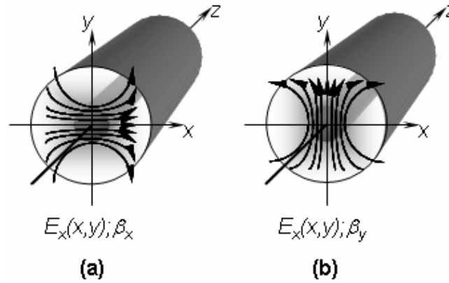
Figure 1 – Two electric field vector polarizations of the HE 11 mode in an optical fibre along the a) x-direction and b) y-direction
