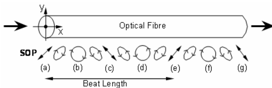
Figure 29 – Relationship between beat length and state of polarization
