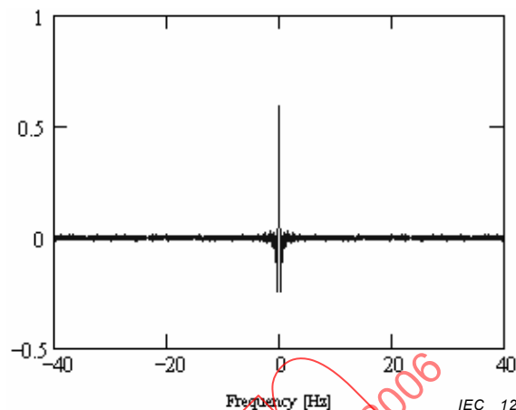
Figure 42 – Frequency spectrum of Figure 41 signal
