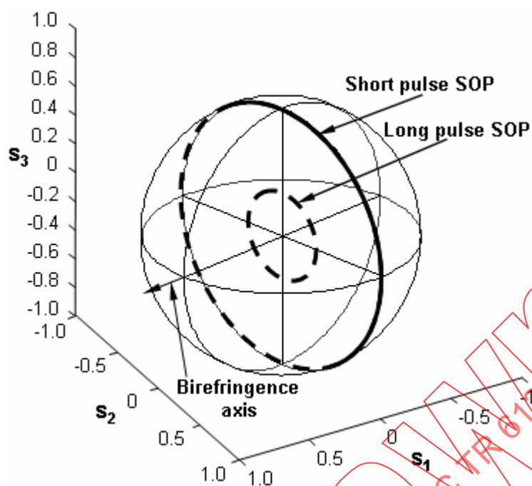
a) For wide SOP-to-birefringence axis angle
