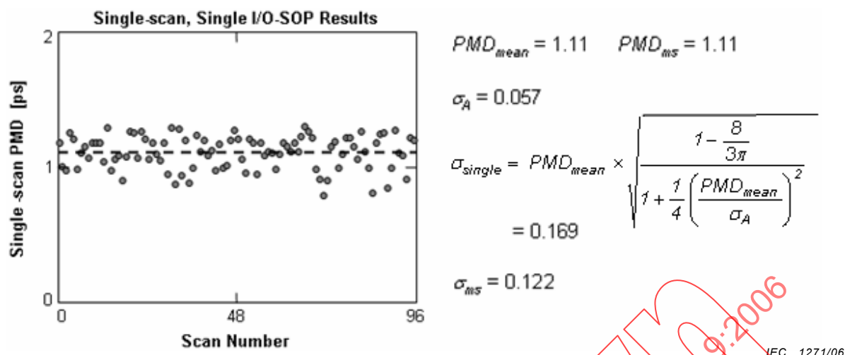
Figure 22 – Comparison between single-scan and scrambling uncertainties
