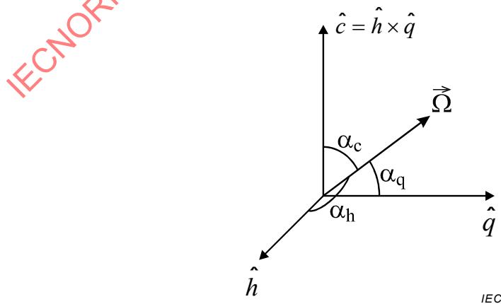
Figure 7 – Relationship of orthogonal output SOPs to the PDV
