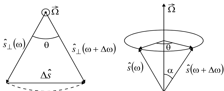
Figure 8 – Stokes vector rotation with frequency change
