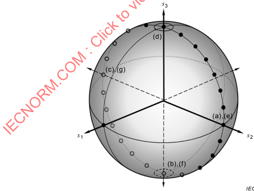
Figure 2 – A rotation on the Poincaré sphere
