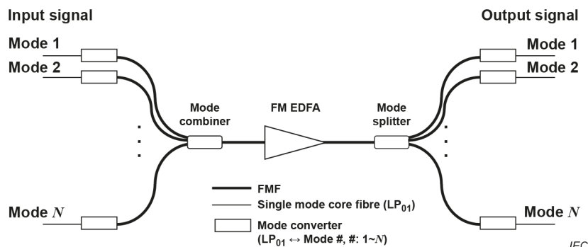
Figure 21 – FM-EDFA evaluation setup for basic optical characteristics
