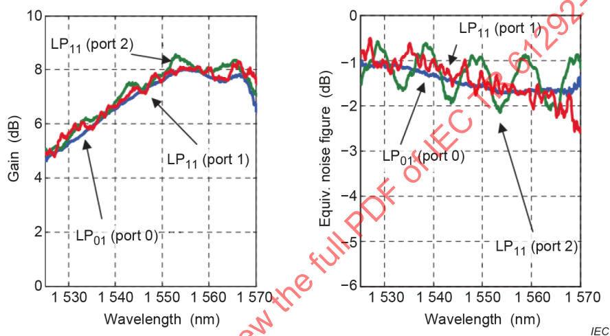
b) On-off gain of Raman amplification and equivalent noise figure at the FME end
