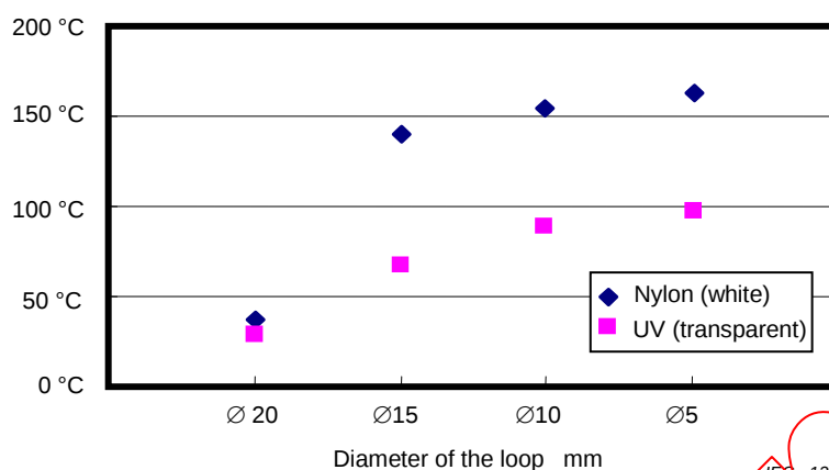
Figure 8 – Temperature of the coating surface of SMFs against bending with optical power of 3 W at 1 480 nm
