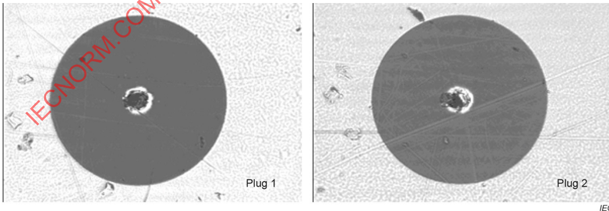
Figure 6 – Polishing surface condition contaminated with metal filing, after test
