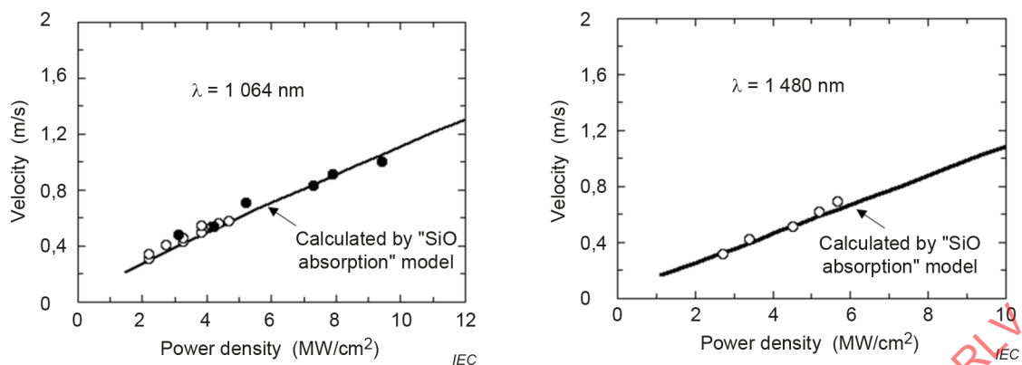
a) Propagation velocity at 1 064 nm wavelength b) Propagation velocity at 1 480 nm wavelength
