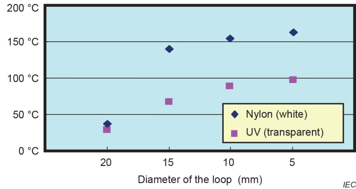
Figure 8 – Temperature of the coating surface of SMFs against bending with optical power of 3 W at 1 480 nm
