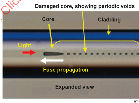
Figure A.1 – Front part of the fibre fuse damage generated in the optical fibre
