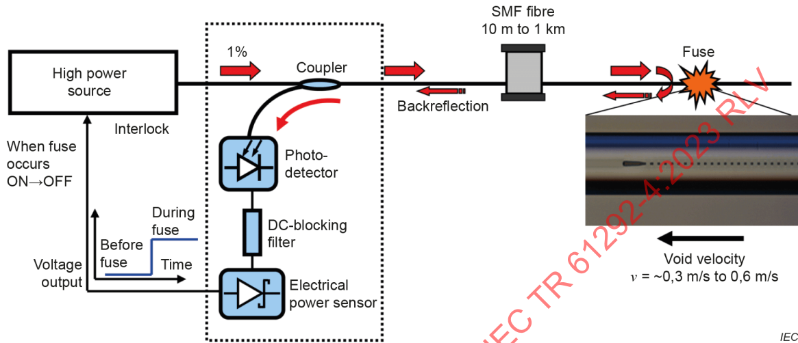
Figure A.10 – Example of fibre fuse active termination scheme
