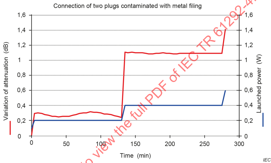
Figure 5 – Variation of power attenuation during test at several power input values for plugs contaminated with metal filings
