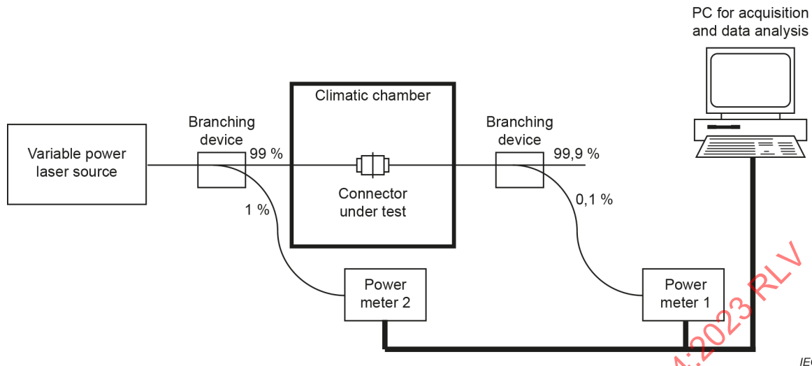
Figure 3 – Test set-up
