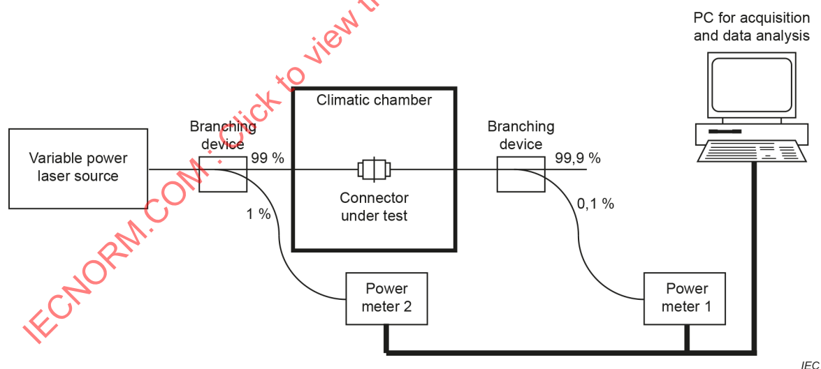
Figure 3 – Test set-up
