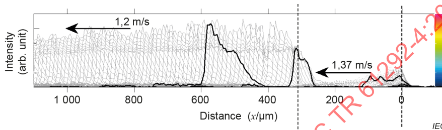
b) Intensity profiles along the dashed lines on the photographs taken every 10 ms
