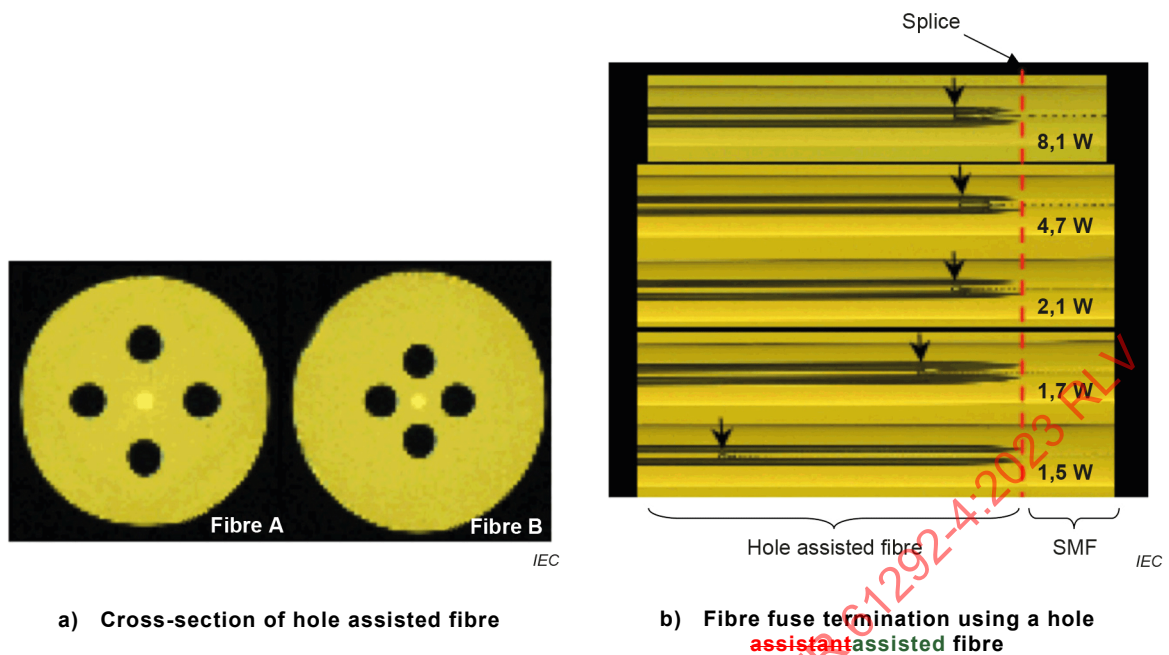
Figure A.9 – Photograph of hole-assisted fibre and fibre fuse termination using a hole-assisted fibre
