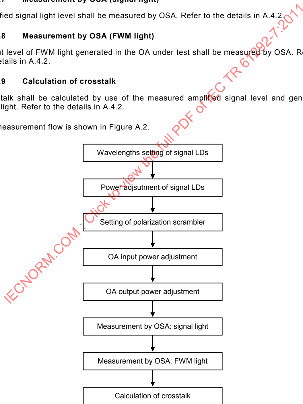
Figure A.2 – Measurement flow chart
