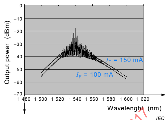
10 c) – SOA chip sample no.3 with a gain ripple of more than 10 dB at I_F = 100 mA
