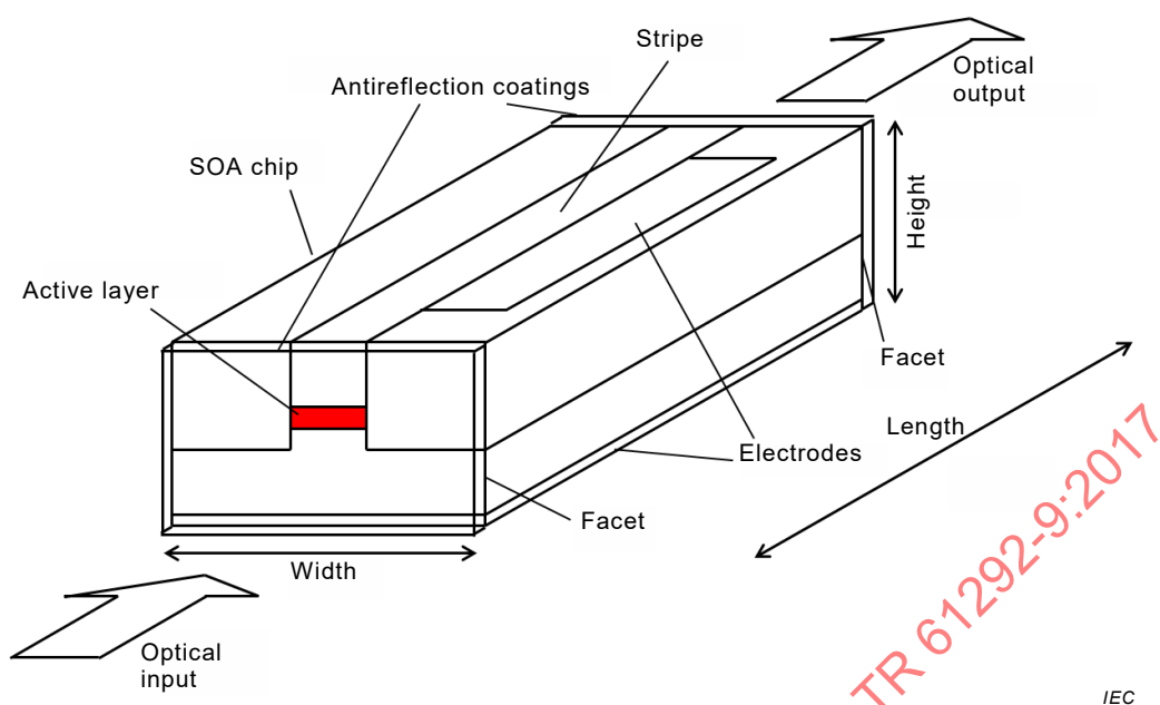
Figure 1 – Schematic diagram of the typical SOA chip
