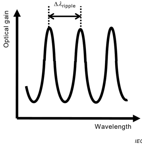
Figure 6 – Schematic diagram of gain ripple
