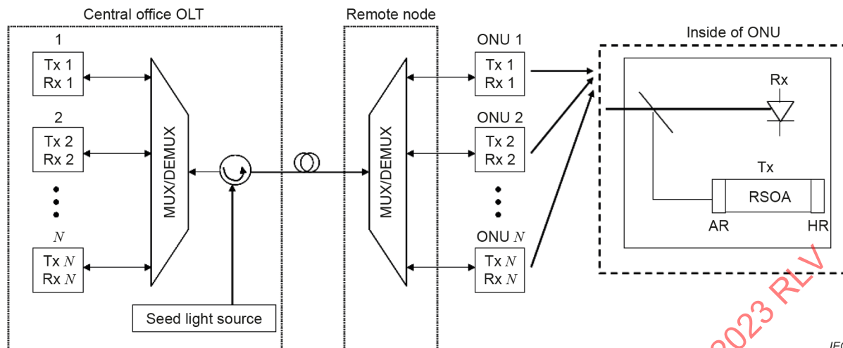
Figure A.3 – Schematic diagram of a seeded WDM-PON system
