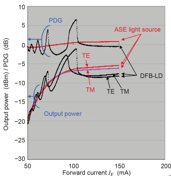
Figure 13 – Output power and PDG of SOA chip sample 3 as a function of I_F
