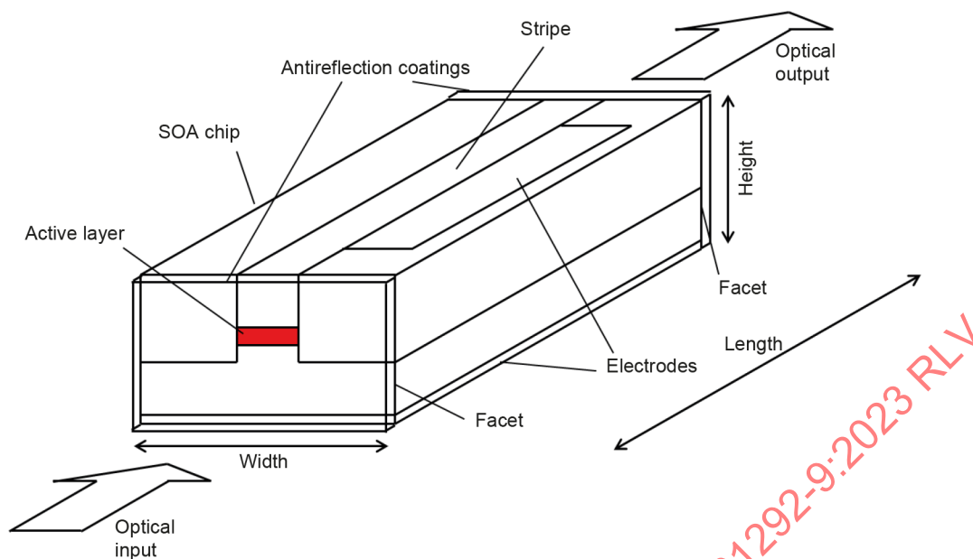
Figure 1 – Schematic diagram of the typical SOA chip
