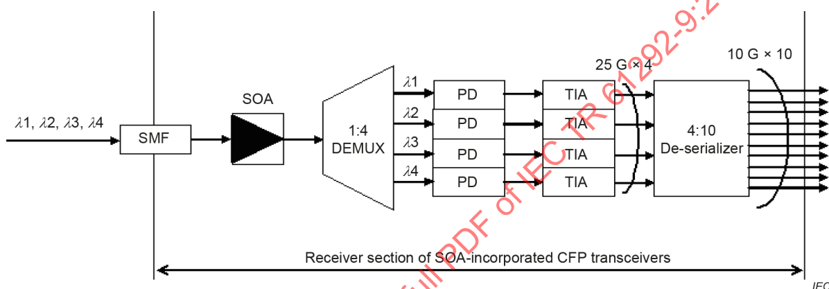
Figure A.1 – Schematic diagram of the receiver section of SOA-incorporated CFP transceivers
