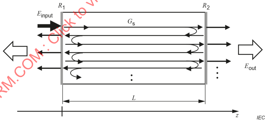
Figure 7 – Illustrated model of a Fabry-Perot type SOA
