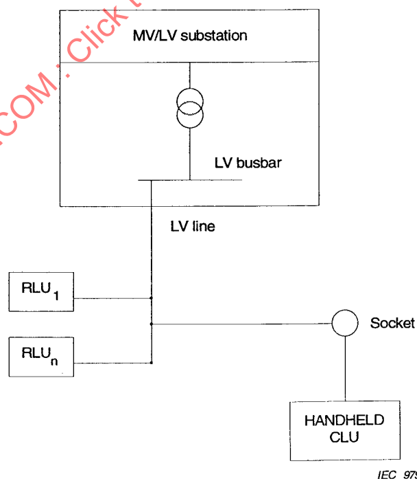
Figure 8 – Local reading via the mains
