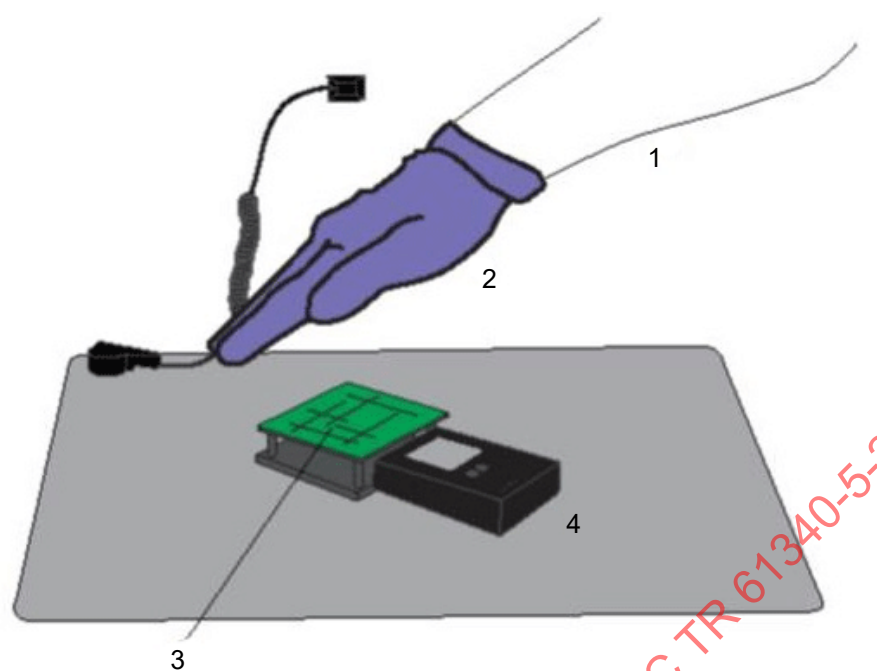
b) – Product charging test using charged plate monitor
