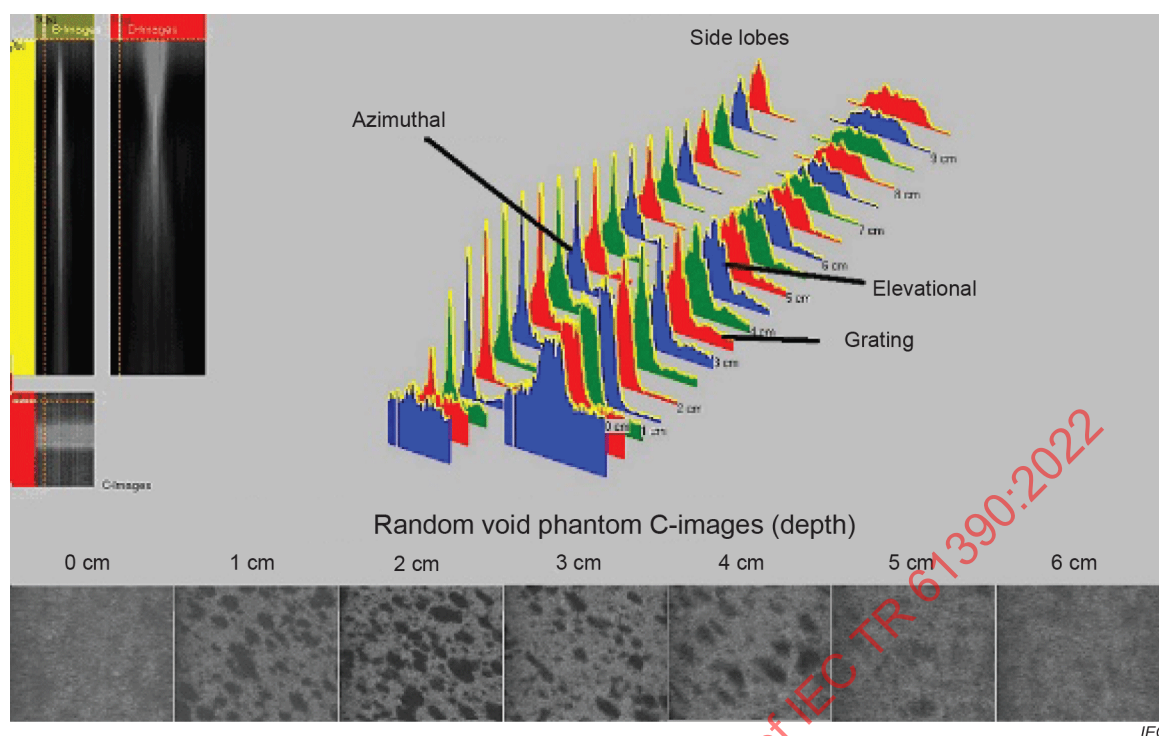
Figure A.15 – (above) Azimuthal and elevational beam profiles obtained from a filament phantom; (below) Constant depth (C-images) from a random-void phantom
