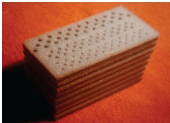
Figure A.8a) Package of TMM slices containing alternating void slices and attenuation slices of polyurethane foam
