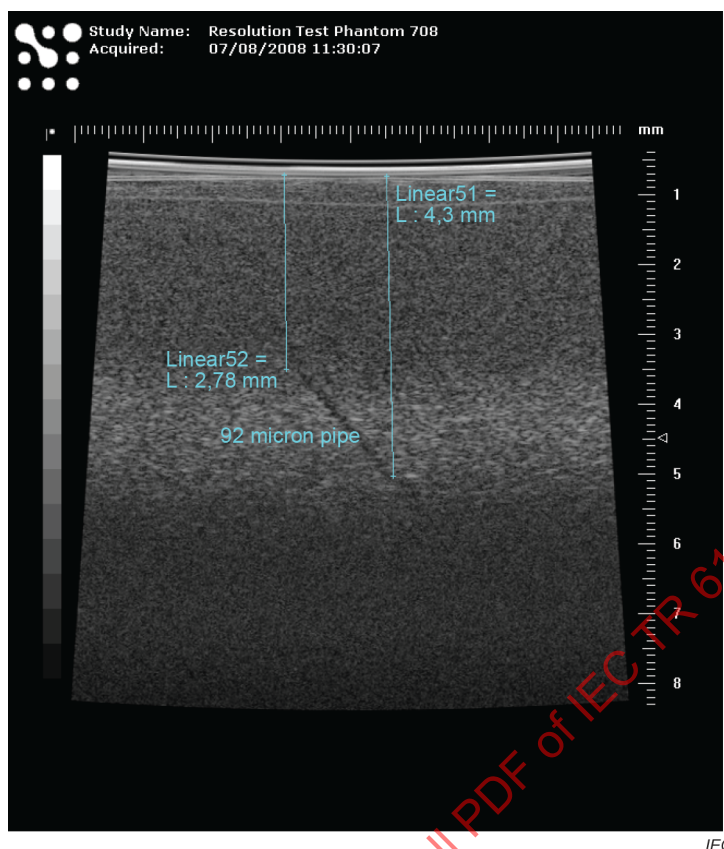
Figure A.11 – Image from a preclinical ultrasound scanner operating at 55 MHz showing the length over which a 92-micron pipe can be visualised in the scan plane
