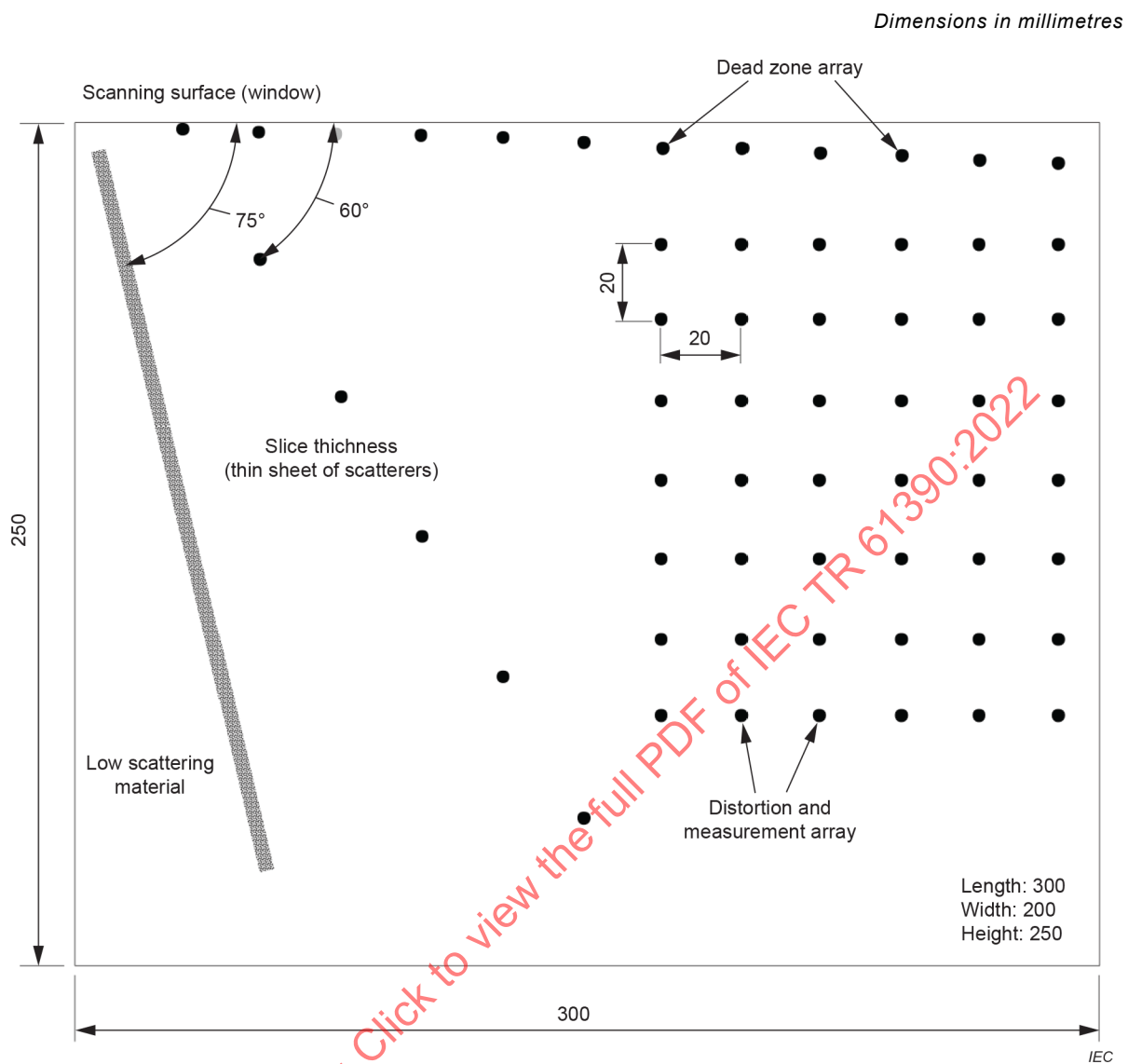
Figure A.3 – Multi-purpose resolution test object
