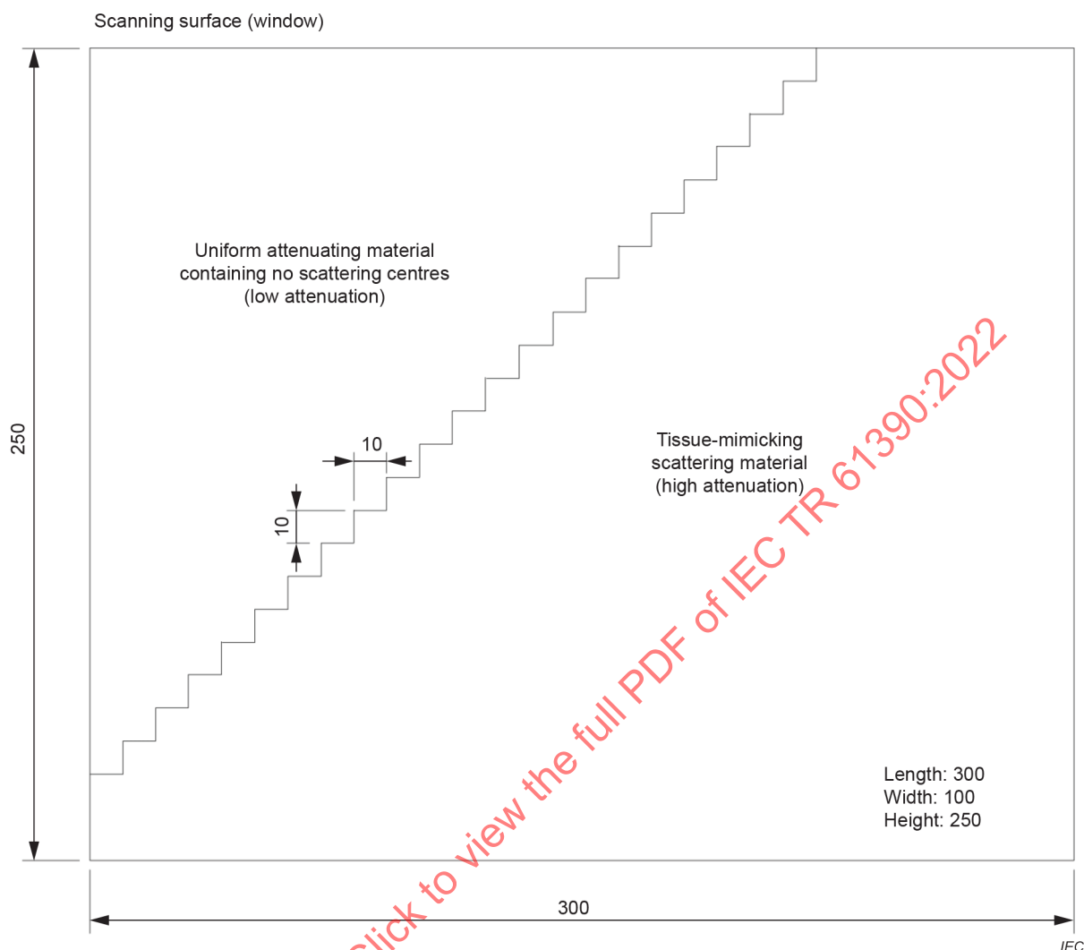
Figure A.1 – Soft tissue-mimicking test object
