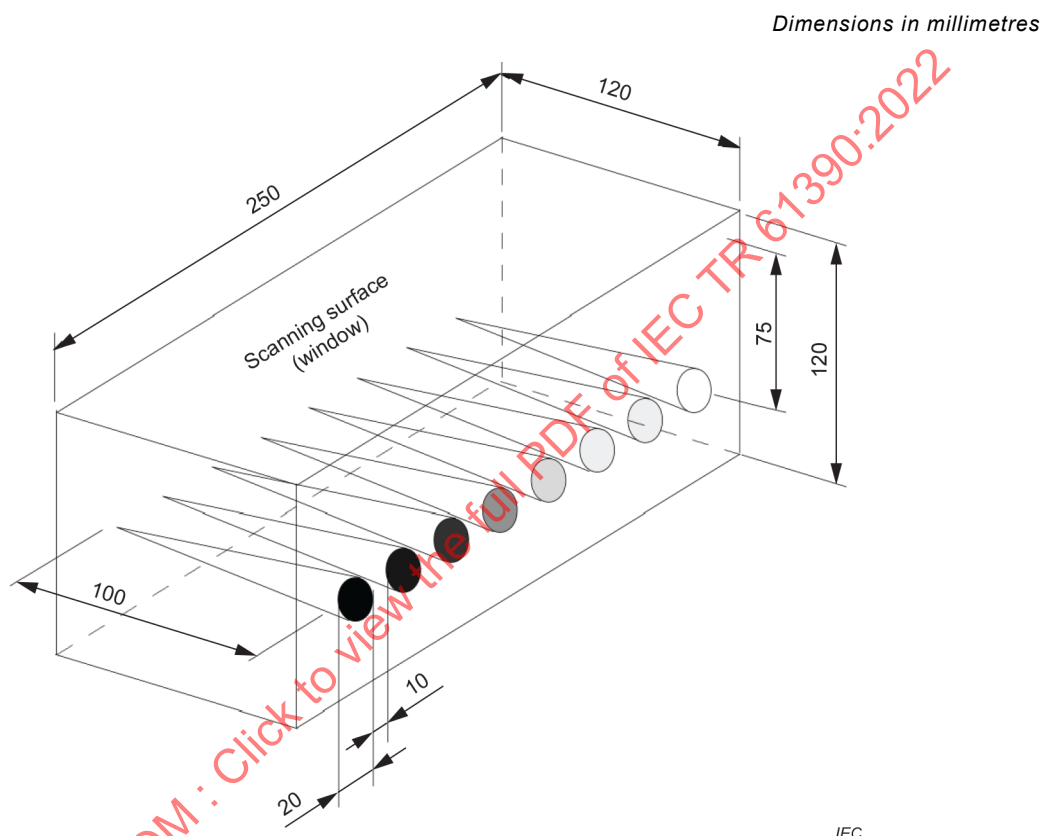
Figure A.5 – Contrast test object
