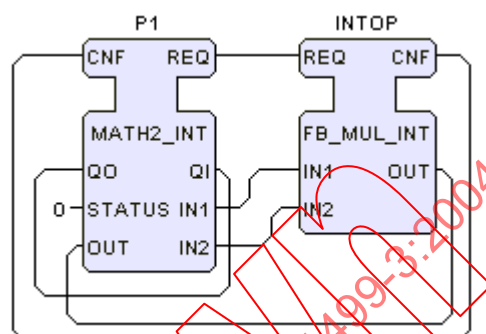
Figure 16b – Multiplication provider body
